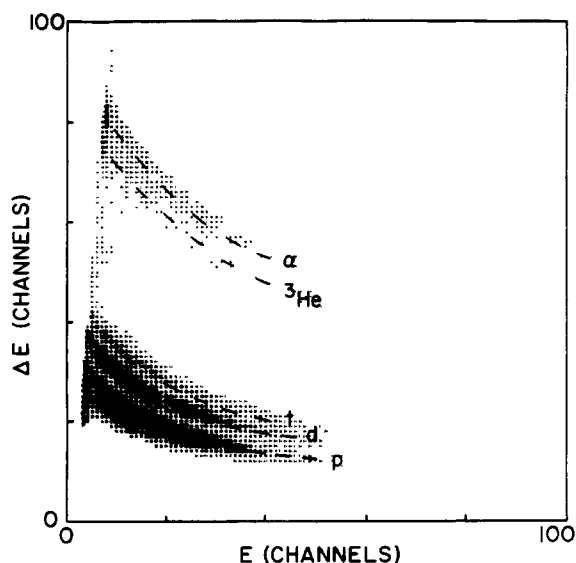
Fig. 11. Contour plot of \Delta E (vertical) vs E (horizontal) for the \text{CaF}_2/\text{plastic} scintillator telescope. The reaction is ^{14}\text{N} + \text{Au} at 35 MeV/A.
