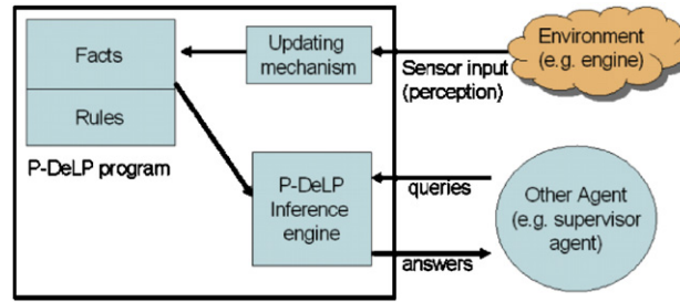
Fig. 2. A P-DeLP-based agent in an MAS context.
