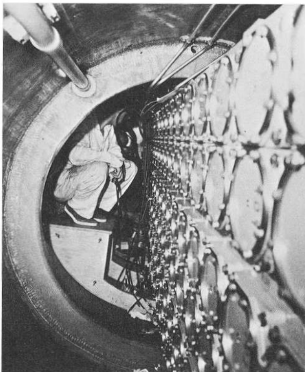
FIG. 5. — A view taken inside the vehicle of the transducer array. During a sonar run the vehicle is flooded and there is a loss of about \frac{1}{2} dB through the vehicle skin on transmission and reception.
