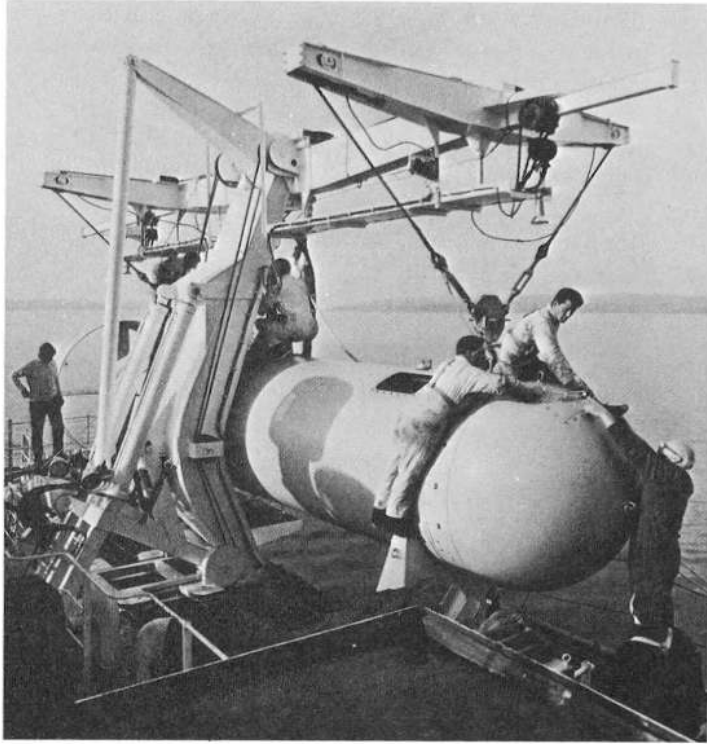
FIG. 6. — The sonar being prepared for a calibration run in Loch Fyne.
