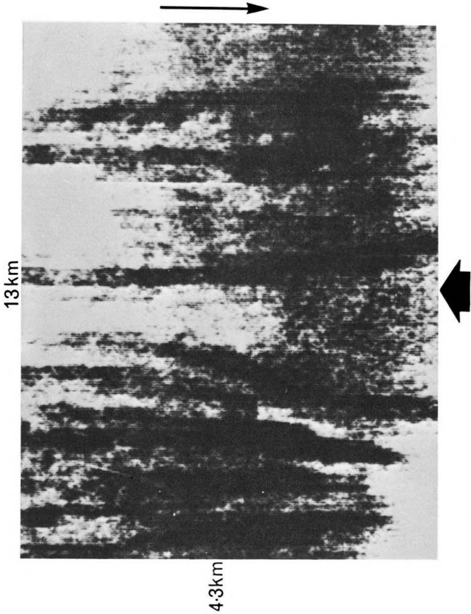
FIG. 12. — A record obtained from part of a survey carried out off the North African coast near Cape Bengut east of Algiers. The range scale is exaggerated by a factor of about 3. The broad arrow gives the direction of 'illumination', and the long thin arrow the downslope direction.
