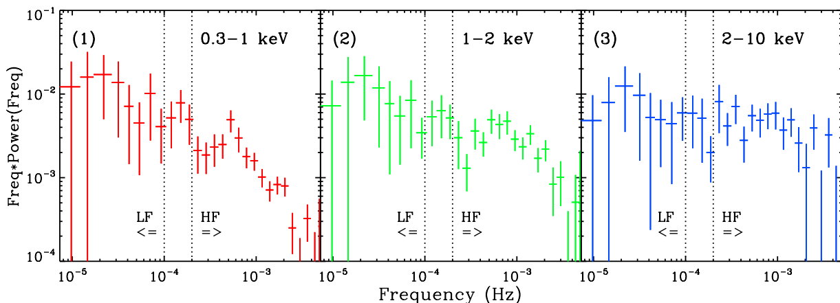
Figure 4. The power spectrum of each energy band after subtracting the Poisson counting noise, calculated by the FTOOL task POWSPEC , rebinned as a geometrical series with geometrical step equal to 1.2.
