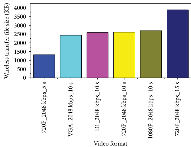
FIGURE 10: Transfer file size in different video formats.
