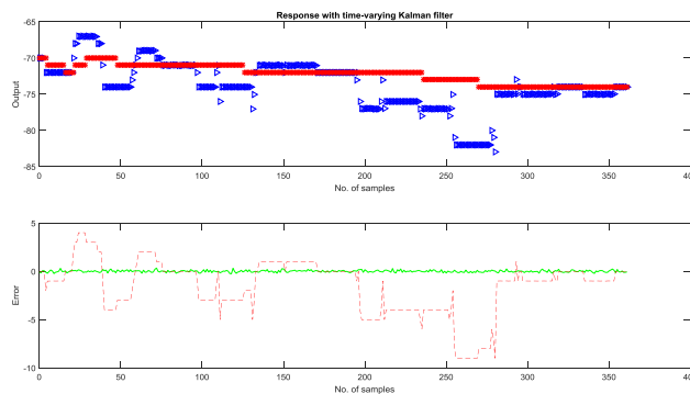
FIGURE 4. Raw RSSI values and RSSI values filtered by Kalman filter (the blue plot is the raw RSSI values while the red plot is the filtered results).
