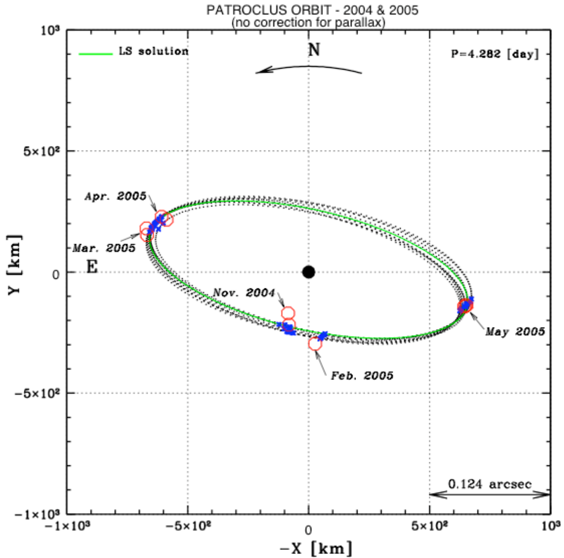
Figure 2 Several good-fit orbits of the 617 Patroclus components estimated using 2004–2005 Keck LGS adaptive optics data. No correction for parallax was made. The LS (Least Square orbit (green) corresponds to the best-fit solution that minimizes the root-mean-square residual. The orbital parameters of the orbit were validated and refined by adding the Gemini/Hokupa’a observations taken in 2001 and 2002. The period is 4.283 days.
