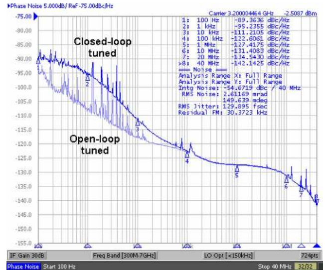
Fig. 15. Measured phase noise for the open-loop and closed-loop tuned PILO (at 3.2 GHz).
