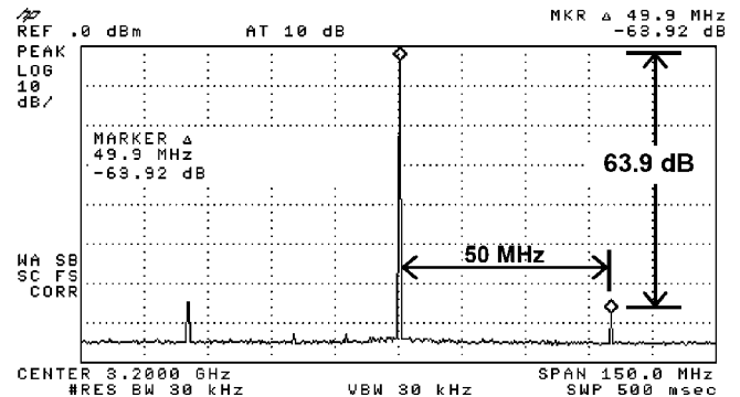
Fig. 16. Measured spurious performance of the close-loop tuned PILO (at 3.2 GHz).
