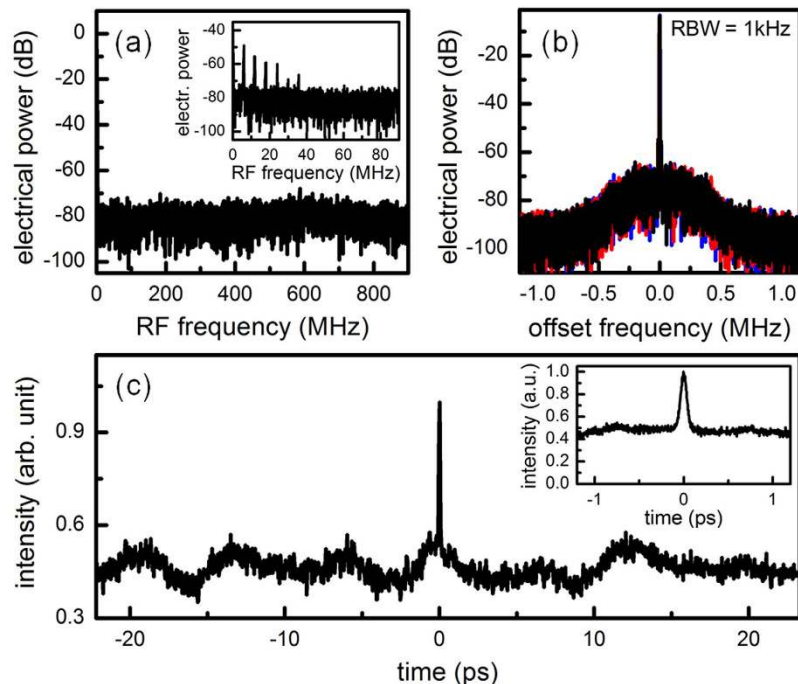
Figure 3. Offset and noise characteristics of the phase-locked 18 GHz comb. (a), RF amplitude noise of the offset-free Kerr frequency comb. Inset: an example RF amplitude noise of the Kerr frequency comb showing multiple peaks due to the beating between different comb families. The comb is tuned to be offset-free by fine control of the pump wavelength. (b), RF spectra of the beat notes from three different filtered spectral regions of the comb (black curve: whole spectrum excluding the pump; blue curve: 1529 to 1538 nm; red curve: 1555 to 1564 nm). All three measurements show bandwidth-limited beat notes at 17.986 GHz, characteristic of a phase-locked comb. The pedestal below 500 kHz offset frequency comes from the local oscillator used for downmixing the 17.986 GHz beat note (Fig. 3). (c), Optical intensity autocorrelation of the phase-locked Kerr frequency comb. The trace has a contrast of \sim 2 , characteristic of a comb without a clean circulating high-power pulse.
