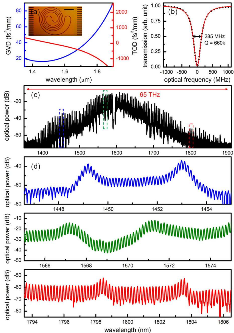
Figure 1. A phase-locked 18 GHz Kerr frequency comb spanning over 65 THz. (a), Simulated group velocity dispersion (GVD) and third order dispersion (TOD) of the ring resonator, featuring small TOD which is beneficial for broad comb generation. Inset: An optical micrograph of the spiral resonator, with a total cavity length of 8.04 mm and a mode area of 1.3 \mu\text{m}^2 . Adiabatic mode converters (the dark bars on the side of the chip) are implemented to improve the coupling efficiency from the free space to the bus waveguide (the bottom straight line across the chip). Scale bar: 250 \mu\text{m} . (b), Example critically-coupled resonant pump mode at 1595.692 nm, with a 285 MHz loaded cavity linewidth. Black dots are the measured data points and the red curve is the fitted Lorentzian lineshape. (c), Example generated Kerr frequency comb, with a broad spectrum spanning nearly half an octave at 65 THz and covering multiple telecommunication bands (E, S, C, L and U bands). (d), Zoom-in views of the comb spectra from 1446.5 nm to 1455 nm (blue), 1565 nm to 1575 nm (green), and 1793.5 nm to 1806.5 nm (red). Even in the wings of the spectrum, native-FSR-spacing comb lines are clearly observed.
