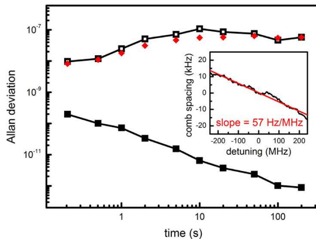
Figure 5. Allan deviation of the free-running (open squares) and the stabilized (closed squares) Kerr frequency comb spacing. In free running mode, the comb spacing stability is limited by the fluctuation resulting from the pump laser wavelength drift (red diamond). Feedback stabilization is achieved by monitoring the comb spacing and controlling the pump laser wavelength to compensate the errors with a proportional-integral controller. Inset: The comb spacing as a function of the pump wavelength detuning, determined at 57 Hz/MHz in our microresonator.
