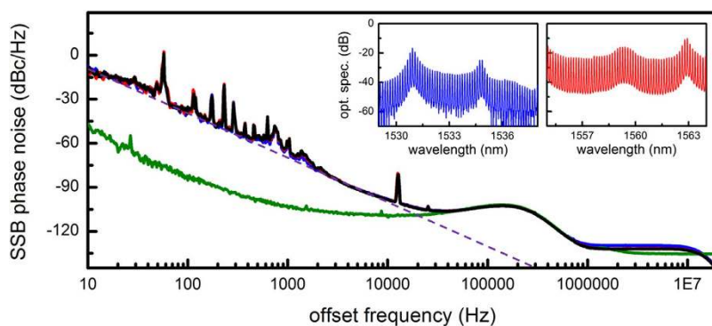
Figure 4. Single-sideband (SSB) phase noises of the beat notes from different spectral regions of the comb. Three filtered spectral regions of the comb with the comb lines are shown in the inset (blue curve: 1529 to 1538 nm; red curve: 1555 to 1564 nm). The black curve shows the whole spectrum excluding the pump. All SSB phase noise spectra show a very low phase noise floor of -130 dBc/Hz at 1 MHz offset from the carrier. For offset frequency below 10 kHz, the phase noise has a roll-off of 30 dB/decade (purple dashed line). The olive curve is the SSB phase noise of the local oscillator used for downmixing the 17.986 GHz beat note.
