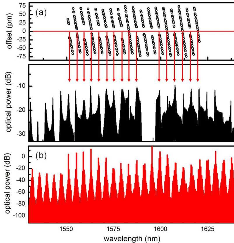
Figure 2. Mode interaction induced spectral modulation of the Kerr frequency comb. (a), Resonance frequency offsets of the second-order mode family with respect to the fundamental mode family (top) as well as the zoom-in view of the Kerr frequency comb (bottom). (b), Simulated Kerr frequency comb by solving the Lugiato-Lefever equation, also showing a 4-nm periodic spectral modulation when the local dispersion disruptions are included in the model.
