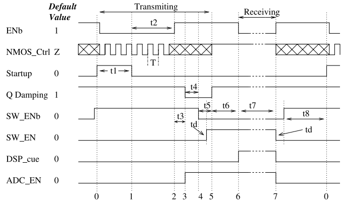
Fig. 10. Simplified control logic waveforms.
