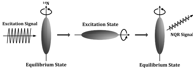
Fig. 1. Illustration of NQR signal excitation.
