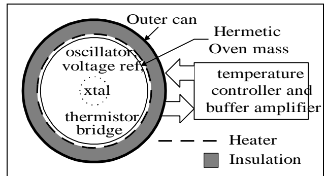
Figure 2. Oscillator partitioning.
