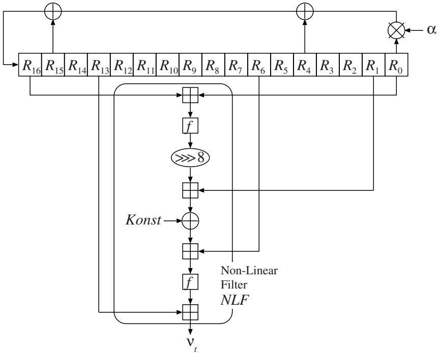
Fig. 1. The structure of non-linear filter NLF
