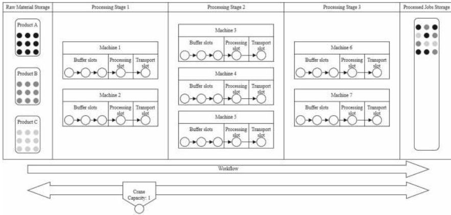
Fig. 1 Exemplary configuration of the shop floor
