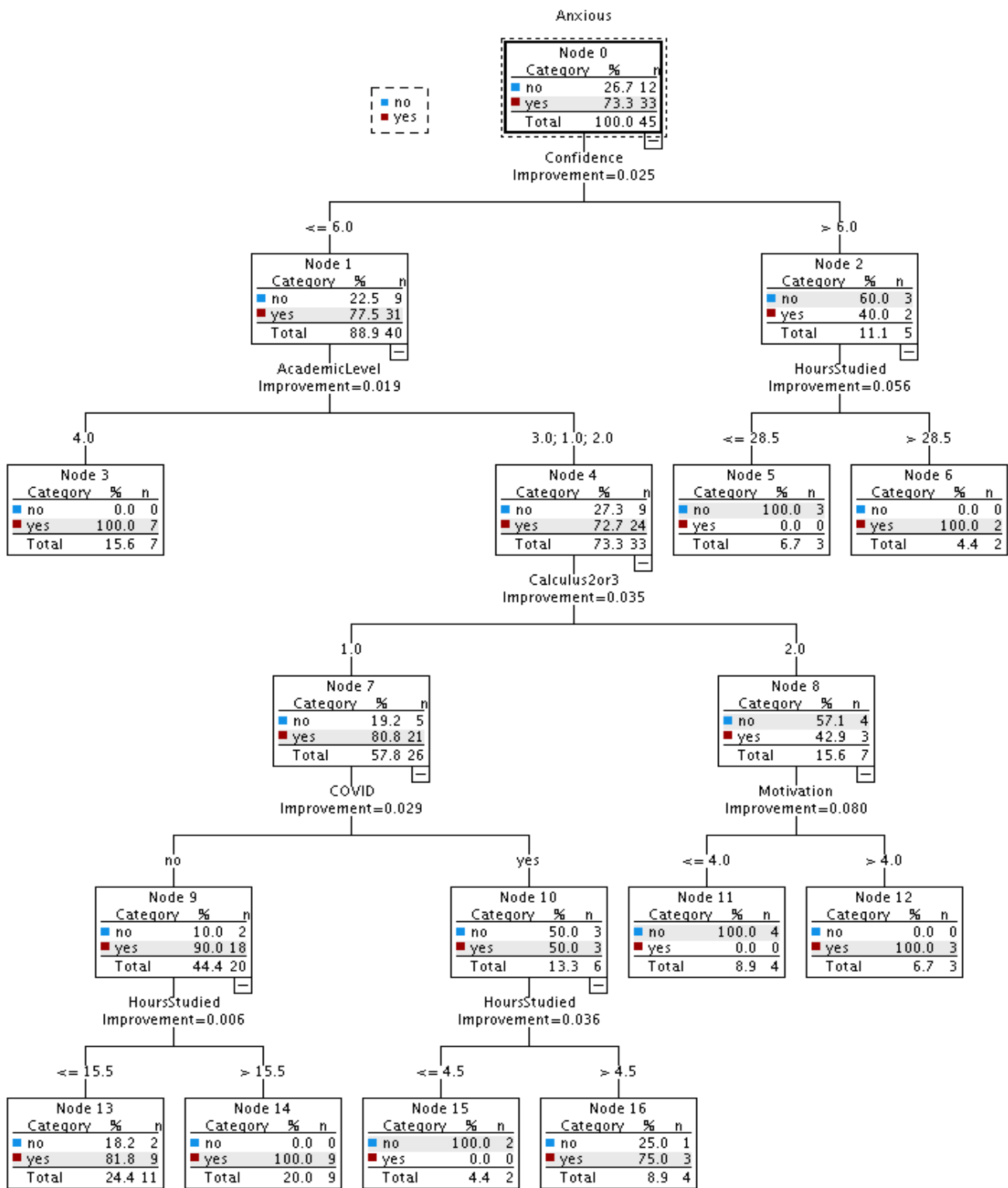
Figure 3. The output tree diagram of the CRT model fitted to survey data of the third week
