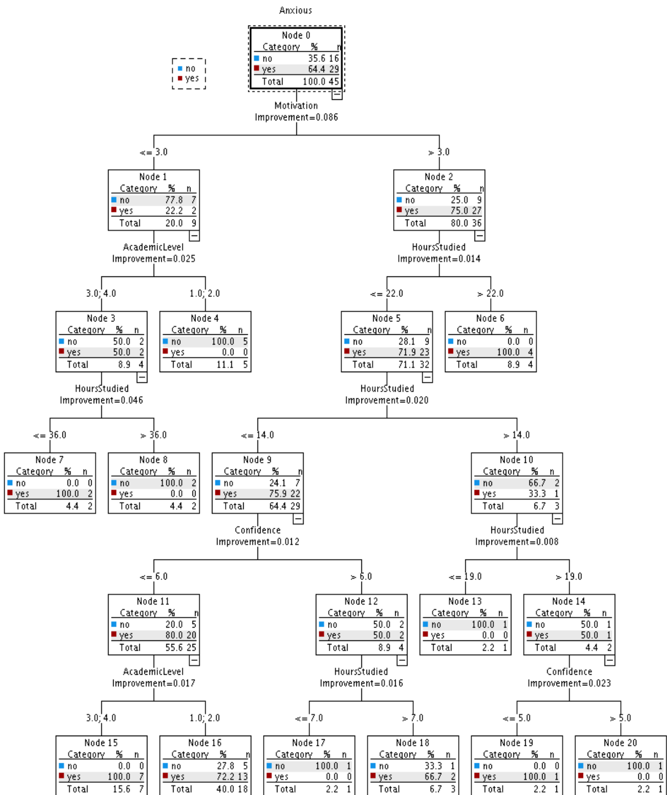
Figure 2. The output tree diagram of the CRT model fitted to survey data of the second week
