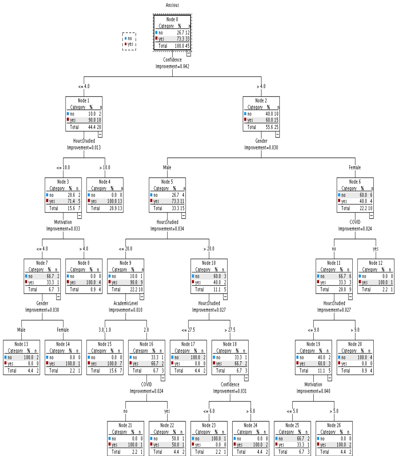
Figure 6. The output tree diagram of the CRT model fitted to survey data of the sixth week
