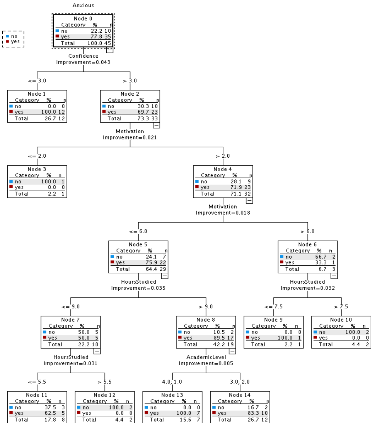
Figure 7. The output tree diagram of the CRT model fitted to survey data of the seventh week
