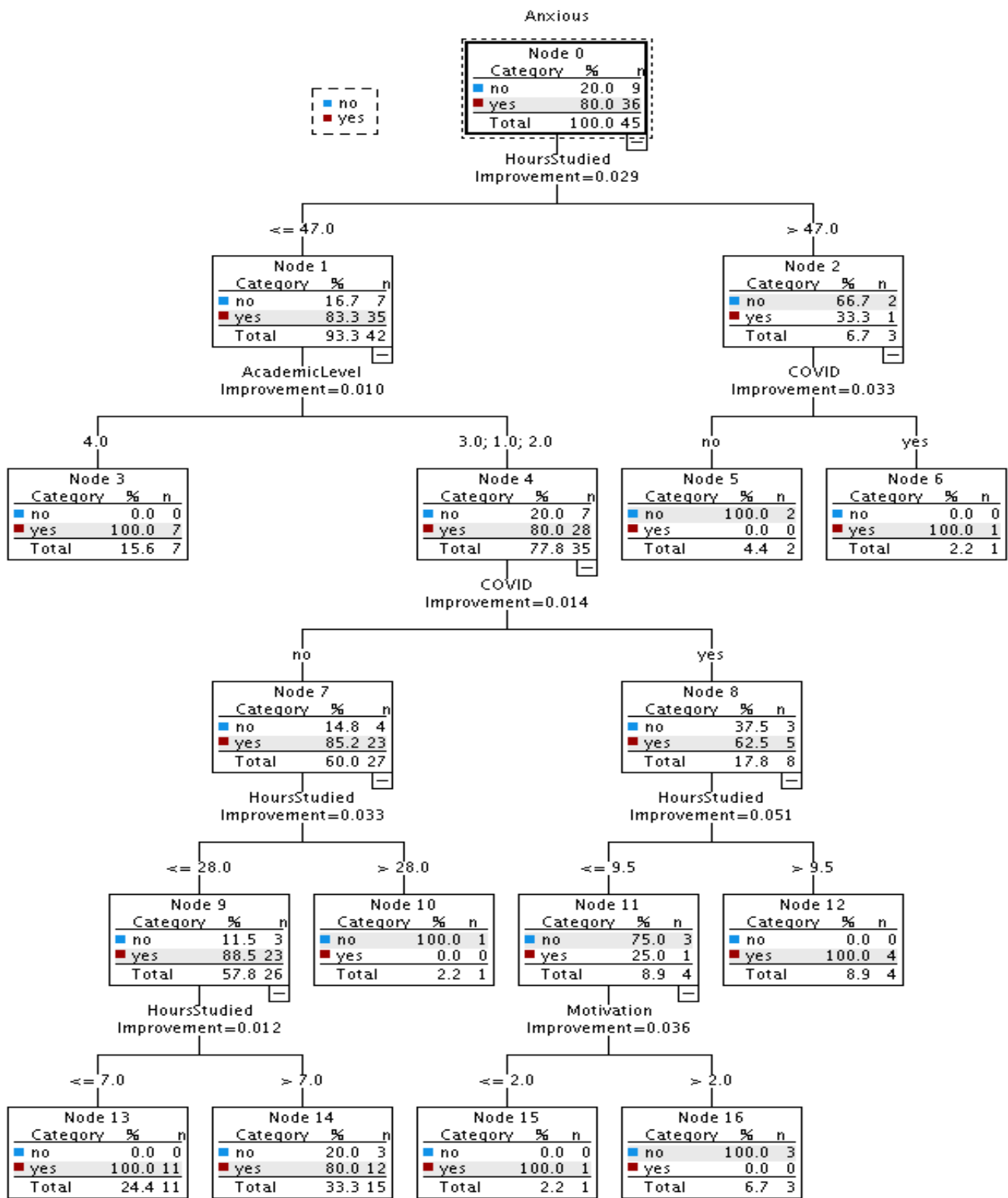
Figure 4. The output tree diagram of the CRT model fitted to survey data of the fourth week
