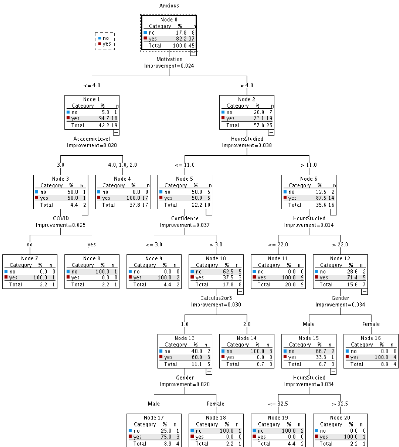
Figure 8. The output tree diagram of the CRT model fitted to survey data of the eighth week
