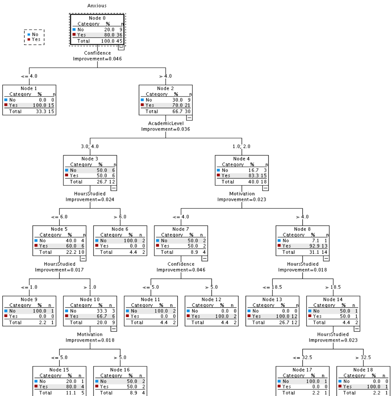
Figure 1. The output tree diagram of the CRT model fitted to survey data of the first week
