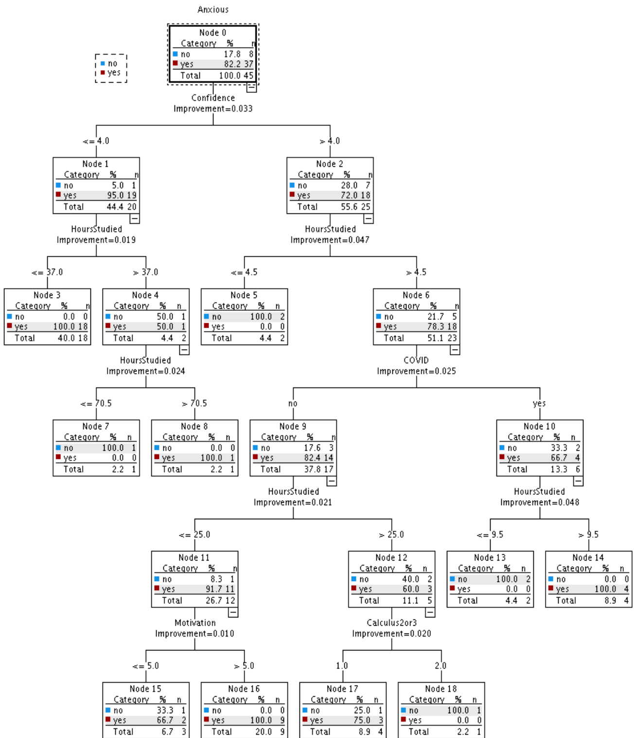
Figure 9. The output tree diagram of the CRT model fitted to survey data of the ninth week
