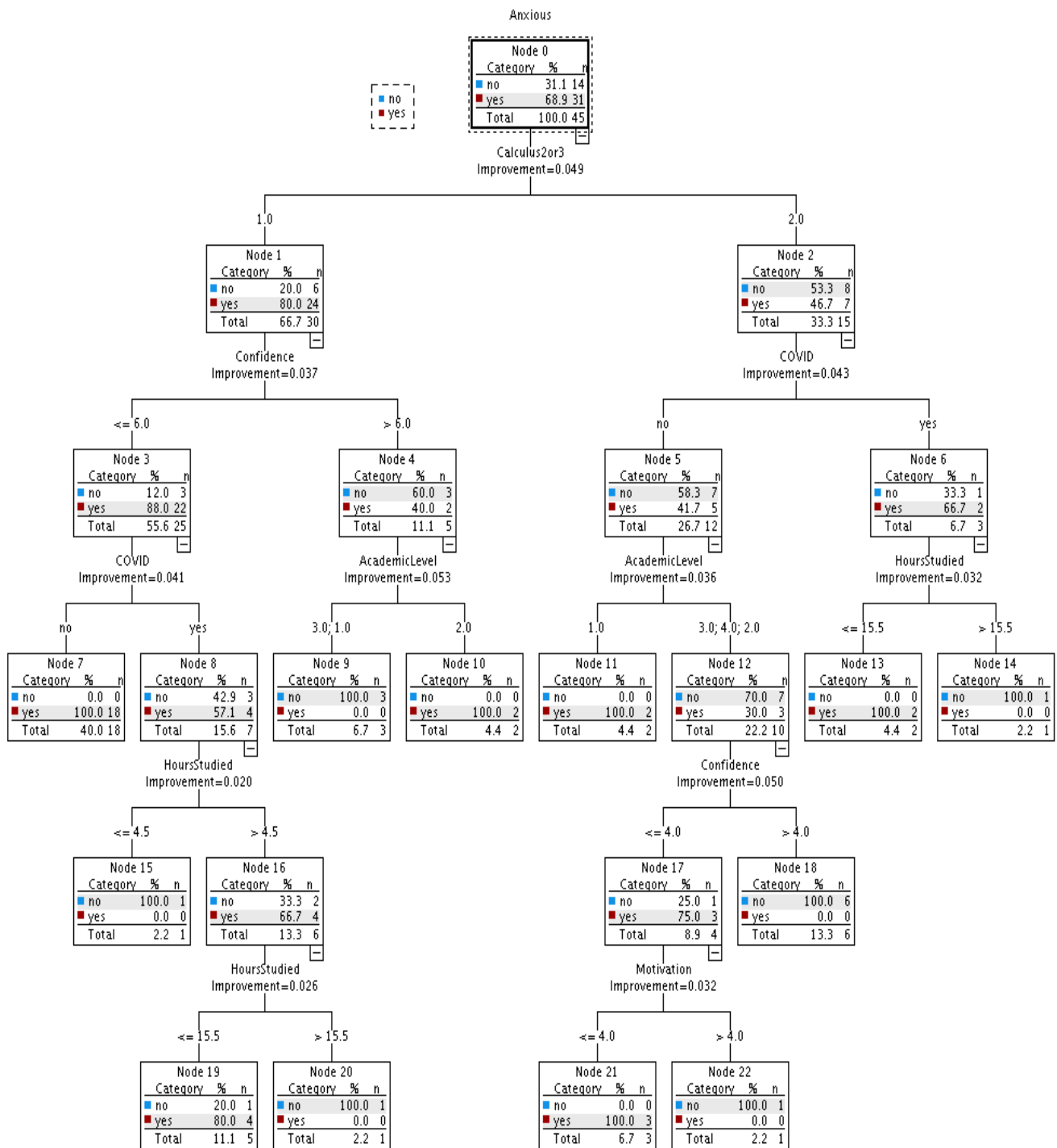
Figure 5. The output tree diagram of the CRT model fitted to survey data of the fifth week
