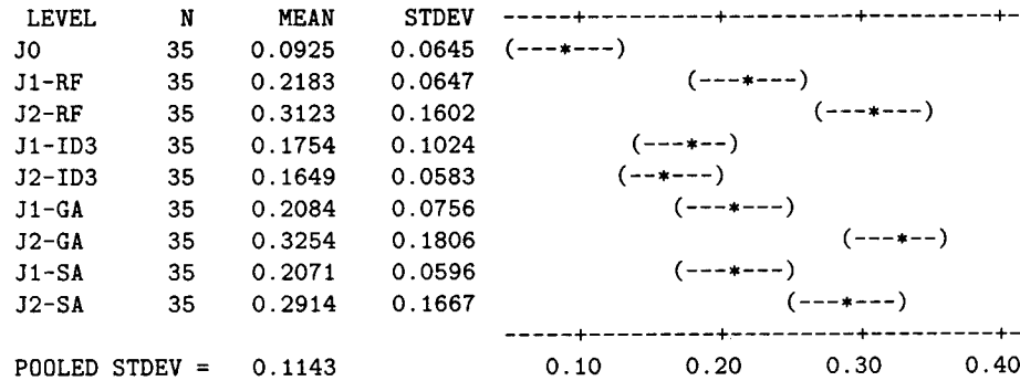
FIG. 2. Results for SMALL test cases.
