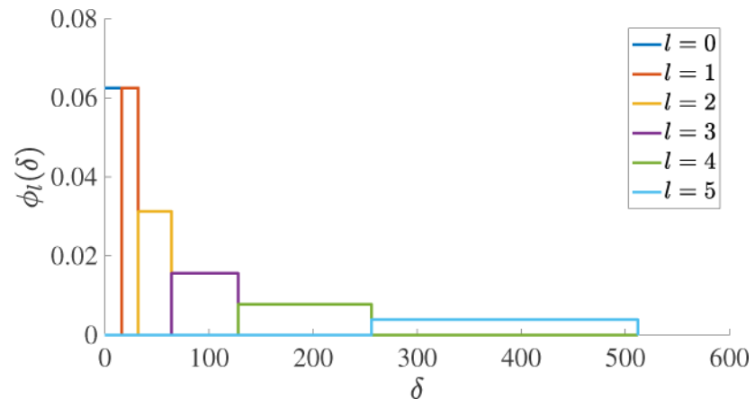
Figure 2. Dyadic influence functions for S = 512 and L = 6 .
