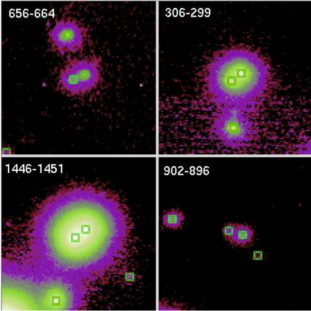
Fig. 15. Close-up view in the K_{\text{S}} band image of the four closest pairs of Table 5. The displayed regions are 6'' \times 6'' and the separations are all in the range of 0.24'' – 0.30'' . Their identifiers as given in Table 3 are overlaid on the images.
