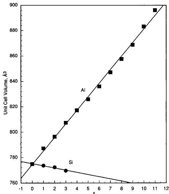
FIG. 2. The 295 K unit cell volume for the \text{Ce}_2\text{Fe}_{17-x}\text{Al}_x , \blacksquare , and \text{Ce}_2\text{Fe}_{17-x}\text{Si}_x , \bullet , solid solutions as a function of x .
