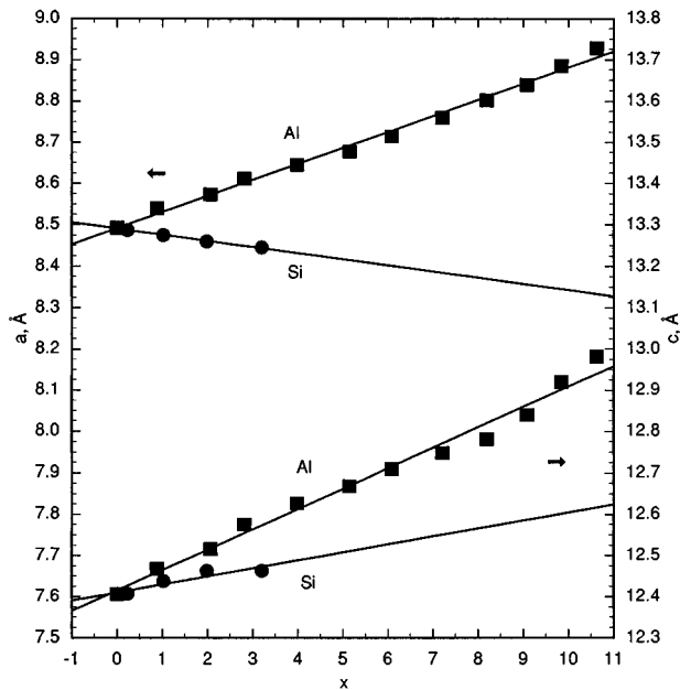
FIG. 1. The 295 K lattice parameters for the \text{Ce}_2\text{Fe}_{17-x}\text{Al}_x , \blacksquare , and \text{Ce}_2\text{Fe}_{17-x}\text{Si}_x , \bullet , solid solutions as a function of x .
