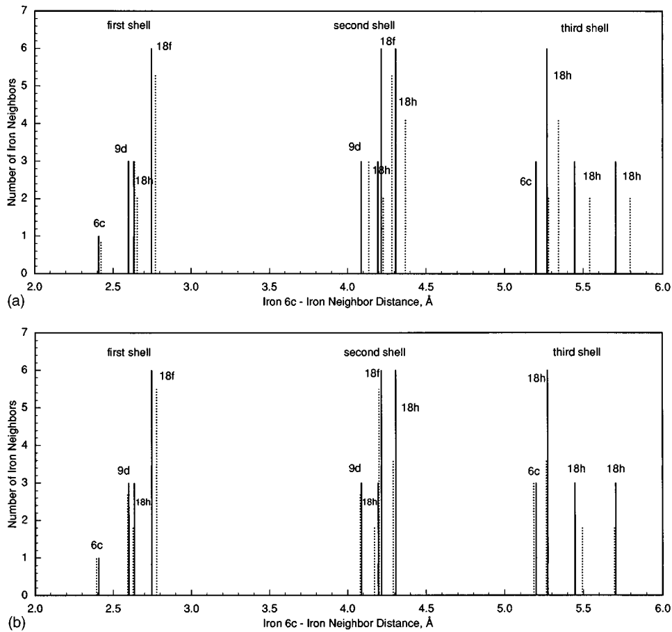
FIG. 13. A plot of the number of iron neighbors for the iron 6c site as a function of distance in Ce_2Fe_{17} , solid lines and Ce_2Fe_{14}Al_3 , dashed lines, A, and Ce_2Fe_{14}Si_3 , dashed lines, B.
