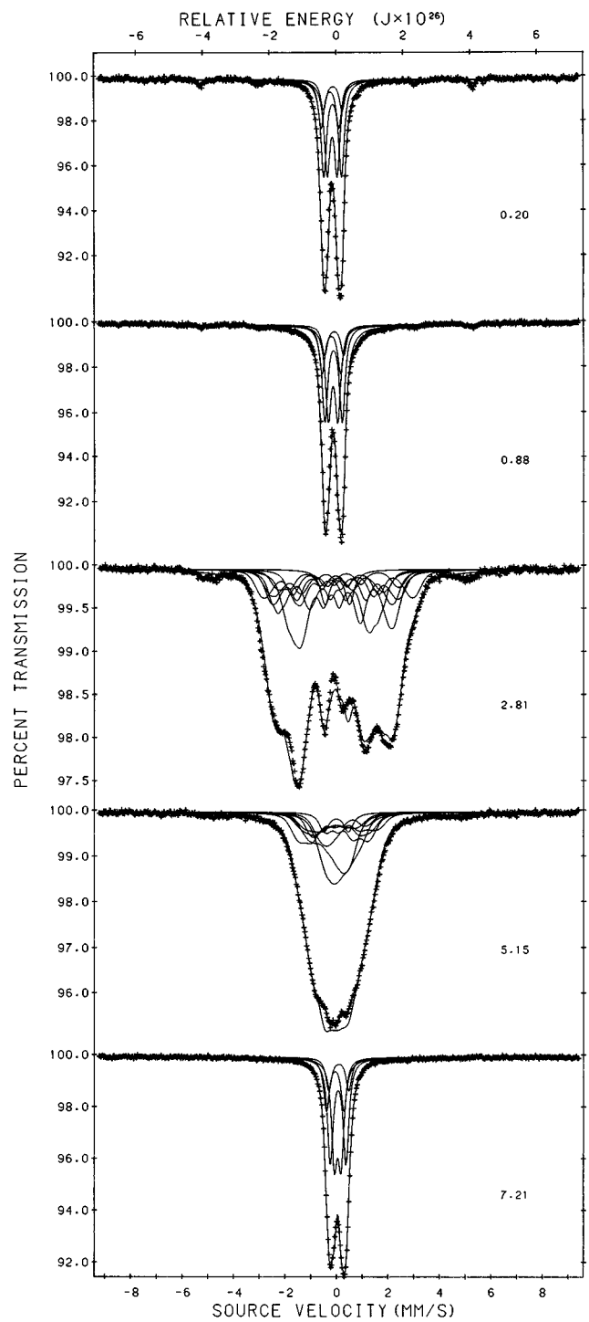
FIG. 8. The Mössbauer spectra of the \text{Ce}_2\text{Fe}_{17-x}\text{Al}_x solid solutions obtained at 295 K.
