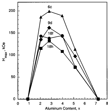
FIG. 9. The maximum hyperfine fields at 295 K for the four iron sites in the \text{Ce}_2\text{Fe}_{17-x}\text{Al}_x solid solutions as a function of aluminum content.
