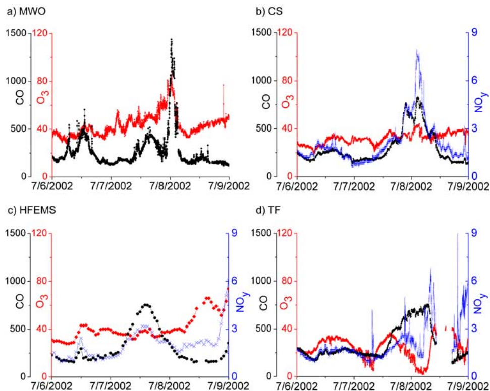
Figure 7. Enhancements in O_3 and NO_y showed a clear altitudinal and latitudinal gradient. Both mixing ratios and R^2 values were greatest at MWO and lowest at TF. CO , O_3 , and NO_y are all displayed in units of ppbv, and dates are given in LT with ticks at 0000.
