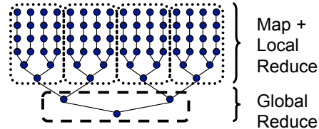
Figure 2: Structuring the Map Reduce
