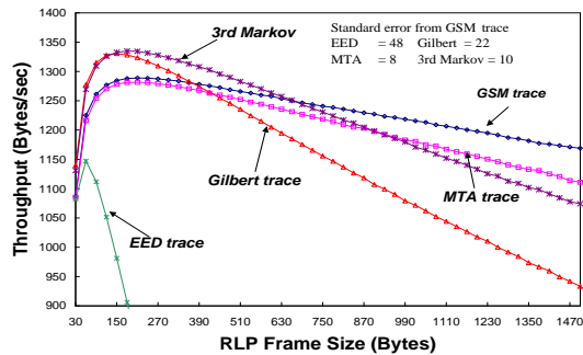
Figure 12. Retrace analysis of four traces.
