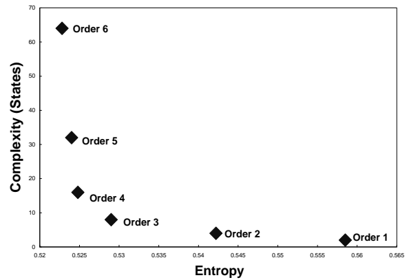
Figure 6. Complexity versus Entropy in lossy trace .
