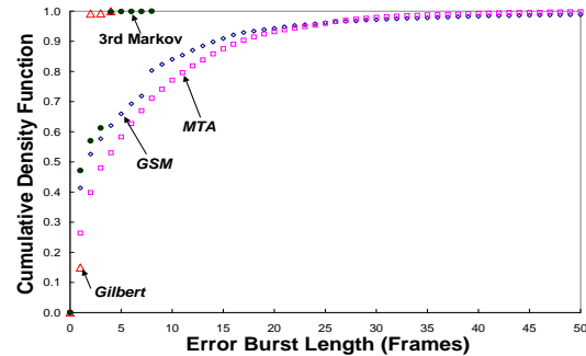
Figure 11. Error burst length distribution.
