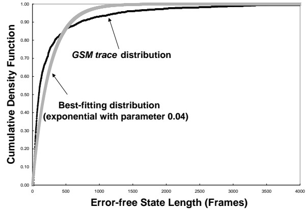
Figure 9. Error-free state length distribution.
