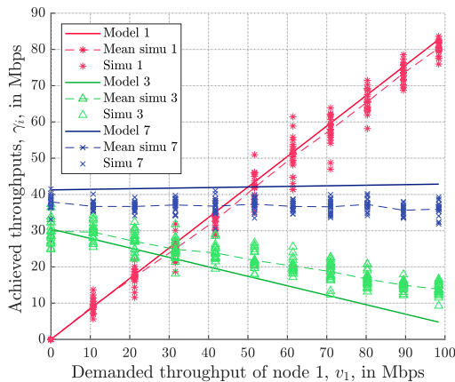
Figure 6: Simulation and model results for the nine-node network of Fig. 5.
