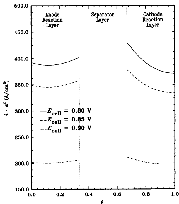
Fig. 5. Variation of the anodic ( i_a \cdot a_a' ) and cathodic ( -i_c \cdot a_c' ) transfer currents for various cell potentials.
