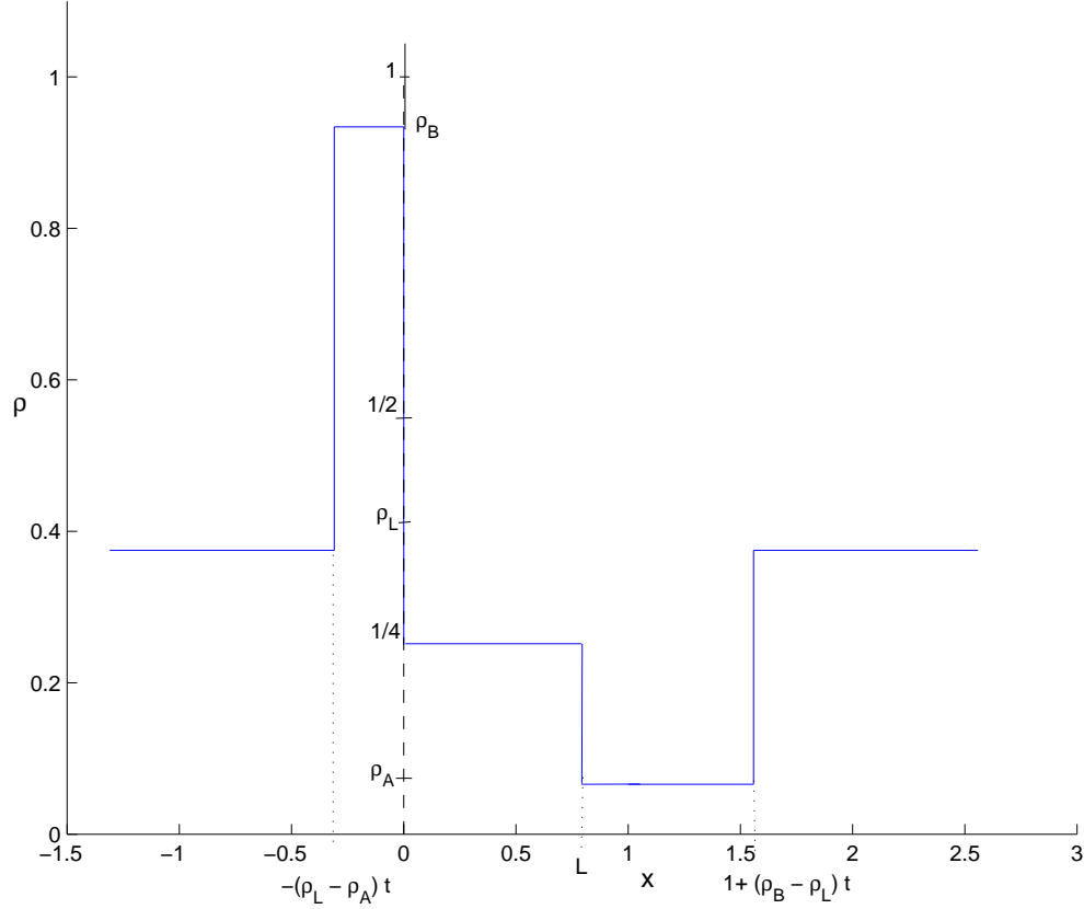
Figure 3: Traffic density profile after the road block has been in place for time t with \rho_L = 3/8 , \lambda = 1/2 and t=1 .
