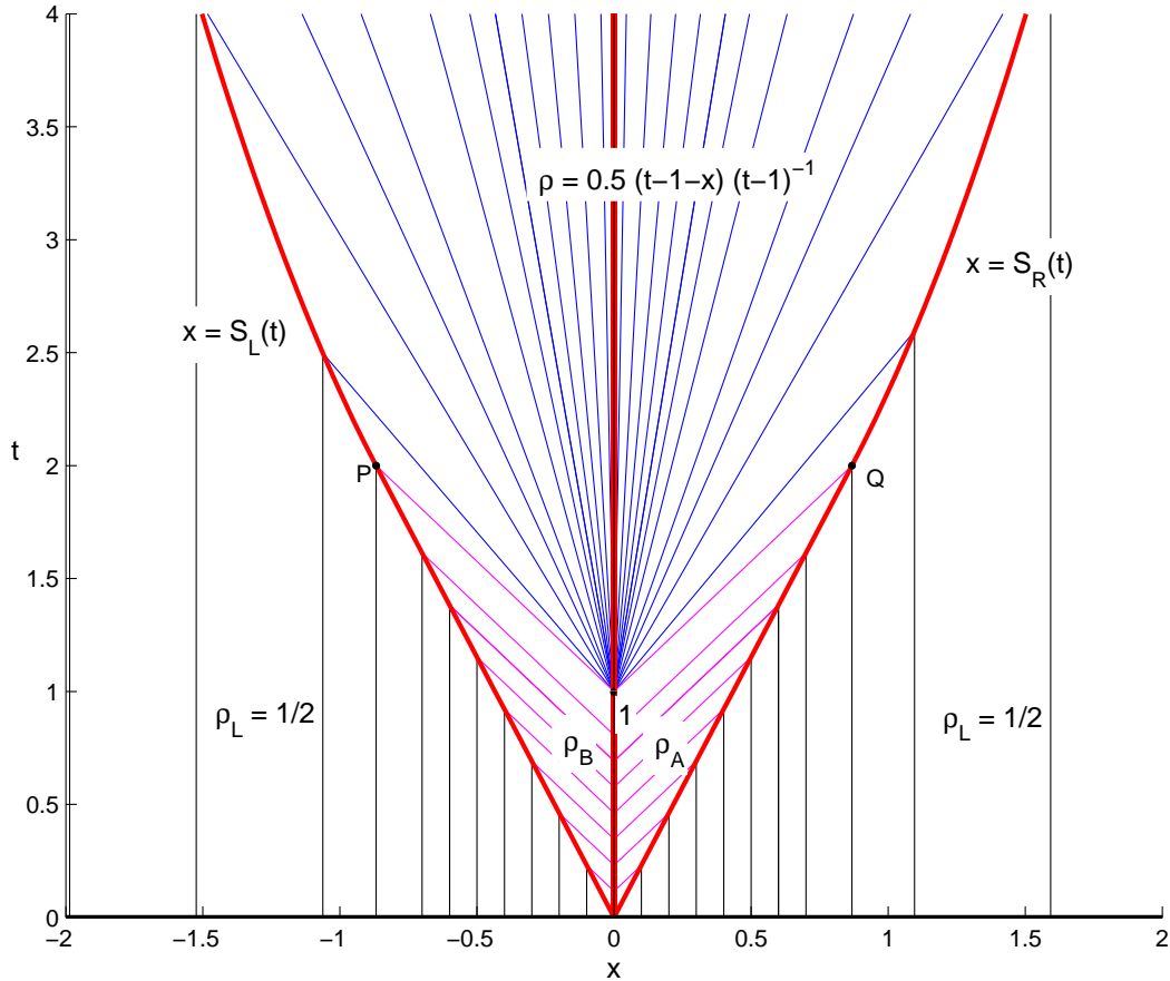
Figure 8: Critical traffic flux. The characteristic projections and shock curves in the (x, t) plane for \rho_L = 1/2 and \lambda = 1/2 .
