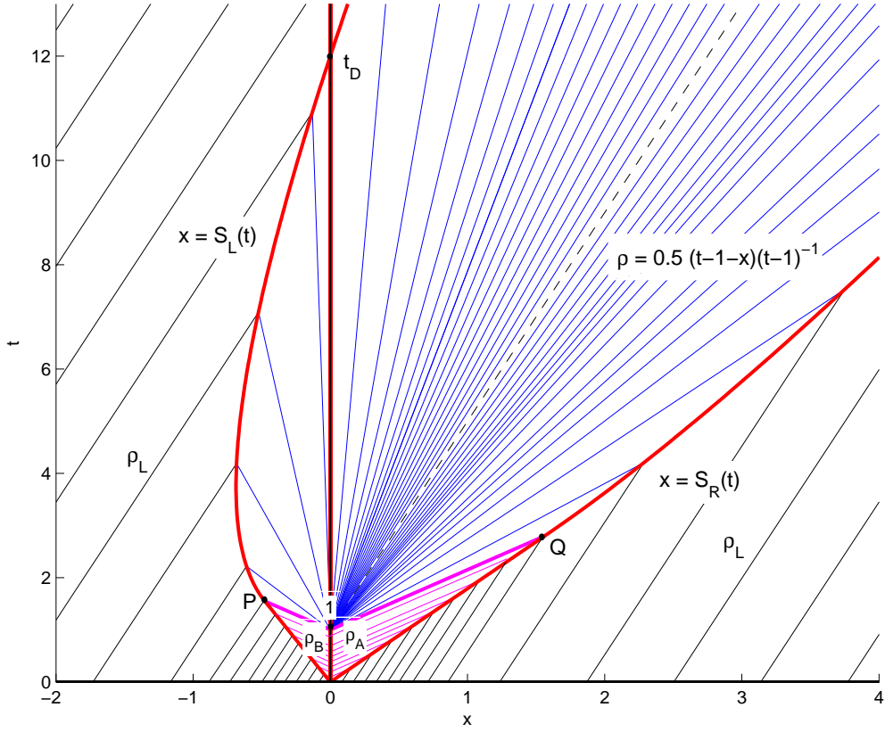
Figure 4: Light traffic. The characteristic projections and shock curves on the (x, t) plane for \rho_L = 3/8 and \lambda = 1/2 . The left shock curve crosses the point x = 0 at t_D = 12 . The dotted line starting at (0, 1) is the dividing characteristic (54).
