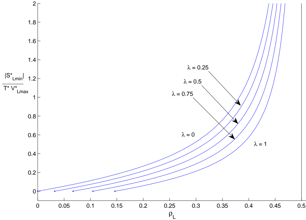
Figure 5: Road block removed. Maximum length of the tailback, scaled by T^* V_{L\max}^* , plotted against the traffic density on the open road \rho_A \leq \rho_L < 1/2 and for a range of values of \lambda .
