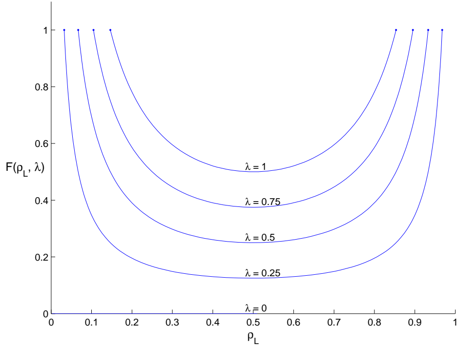
Figure 2: Ratio F(\rho_L, \lambda) of the traffic flux out of the road block to the traffic flux into the left shock plotted against the traffic density on the open road \rho_L for \rho_A \leq \rho_L \leq \rho_B and for a range of values of \lambda .
