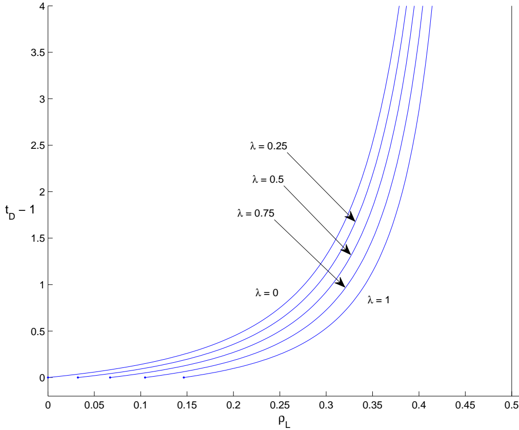
Figure 6: Ratio of the additional time taken for the effects of the road block to clear to the time the road block was in place, t_D - 1 , plotted against \rho_L for \rho_A \leq \rho_L < 1/2 and for a range of values of \lambda .
