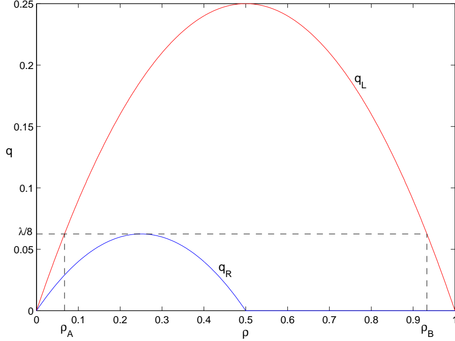
Figure 1: The traffic flux in the open road, q_L , and in the road block, q_R , plotted against the traffic density \rho for \lambda = 1/2 . The traffic densities \rho_A and \rho_B are defined by (10) and (11).
