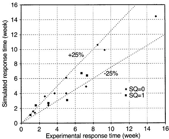
Fig. 8. Comparison of simulated and experimental response times needed for initiation of mould growth on pine sapwood in fluctuating humidity conditions. Values of surface quality SQ correspond to original kiln-dried (1) and resawn (0) surfaces
