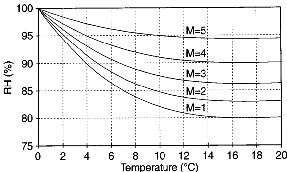
Fig. 2. Temperature-dependent critical relative humidity needed for mould growth at different values of mould index
