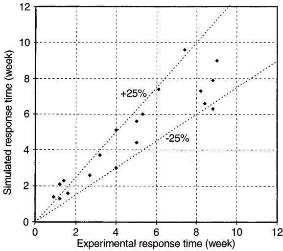
Fig. 5. Comparison of simulated and experimental response times needed for visual appearance of mould growth on pine sapwood in constant conditions
