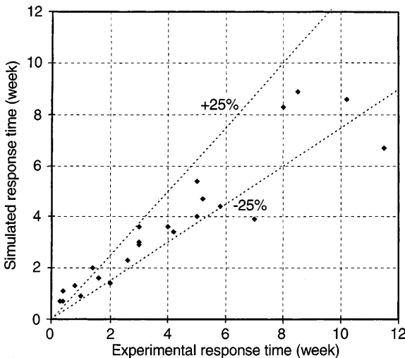
Fig. 4. Comparison of simulated and experimental response times needed for initiation of mould growth on pine sapwood in constant conditions
