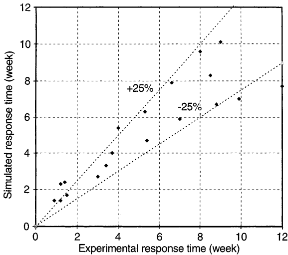
Fig. 7. Comparison of simulated and experimental response times needed for visual appearance of mould growth on spruce sapwood in constant conditions
