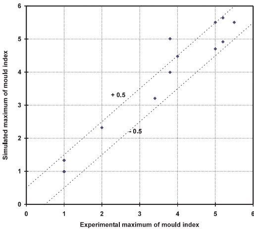
Fig. 3. Comparison of the largest possible value of mould index produced by Eq. (2) against the experimenta
