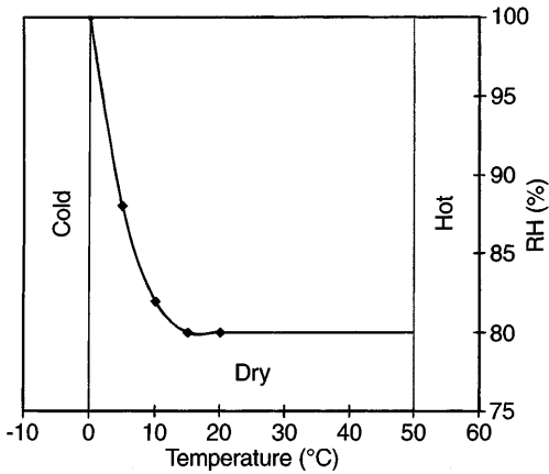
Fig. 1. Conditions favourable for initiation of mould growth on wooden material as a mathematical model
