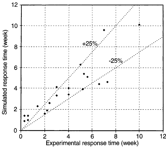
Fig. 6. Comparison of simulated and experimental response times needed for initiation of mould growth on spruce sapwood in constant conditions
