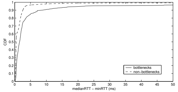
Fig. 15. Bottlenecks vs. queueing delay
