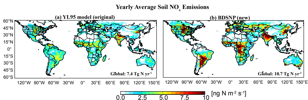
Fig. 1. Comparison of above-soil NO x emission inventories. Emissions calculated from (a) the original YL95 parameterization as implemented into GEOS-Chem (Wang et al., 1998) are compared with (b) the updated model (BDSNP) for the year 2006. Calculated global 2006 emissions are listed (lower right). Color bar saturates at 10 ng N m -2 s -1 .
