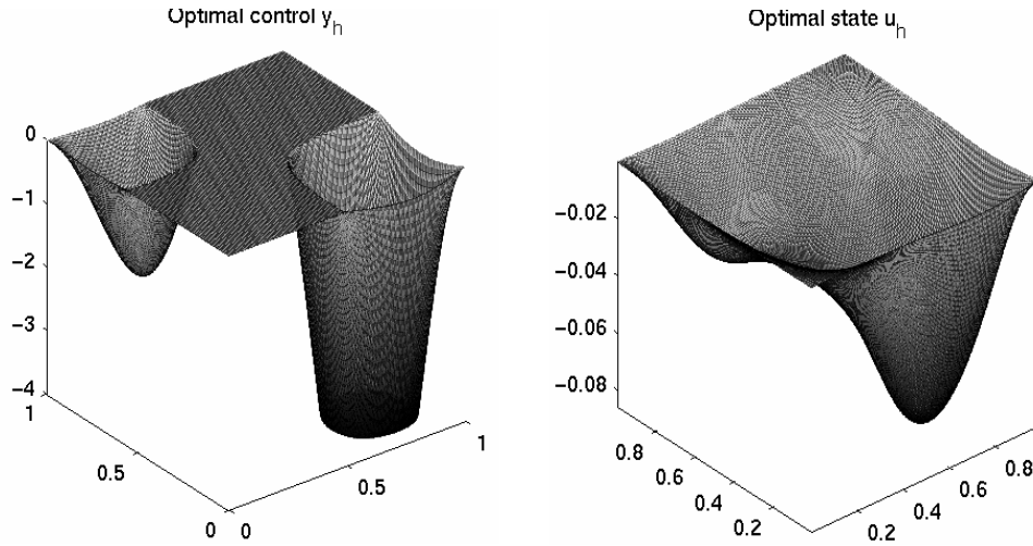
FIG. 6.1. Optimal control and state for h = 1/256 .
