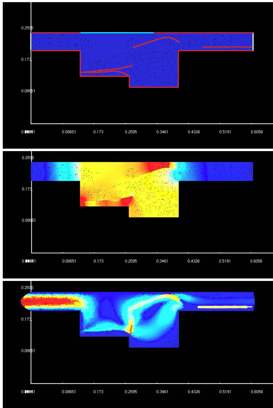
Figure 6. Position of particles and sheets of paper (top), pressure distribution (center) and velocity field (bottom) at t = 0.15 s
