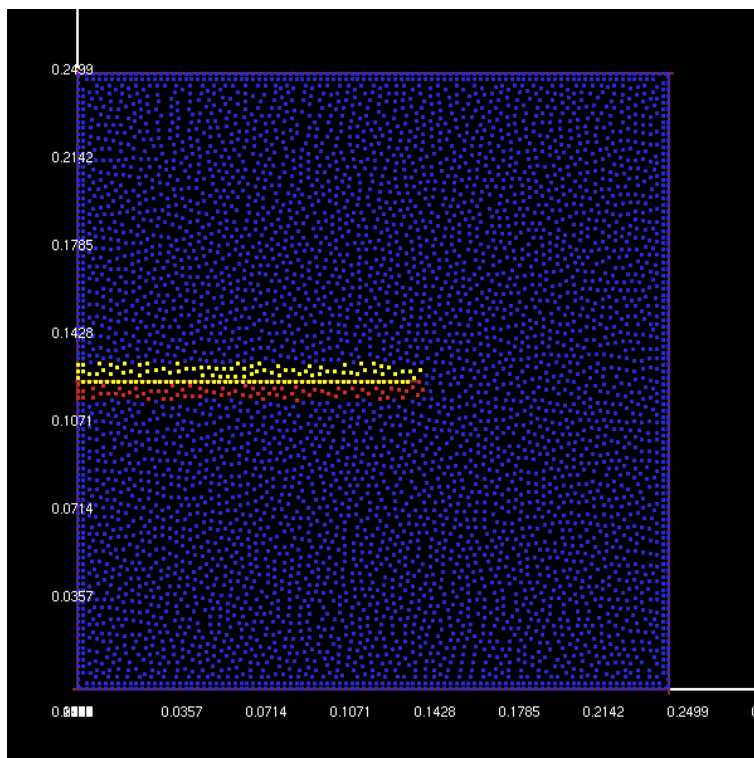
Figure 1. Orientations of the particles around a sheet of paper, blue indicates orientation 0, red +1 and yellow -1
