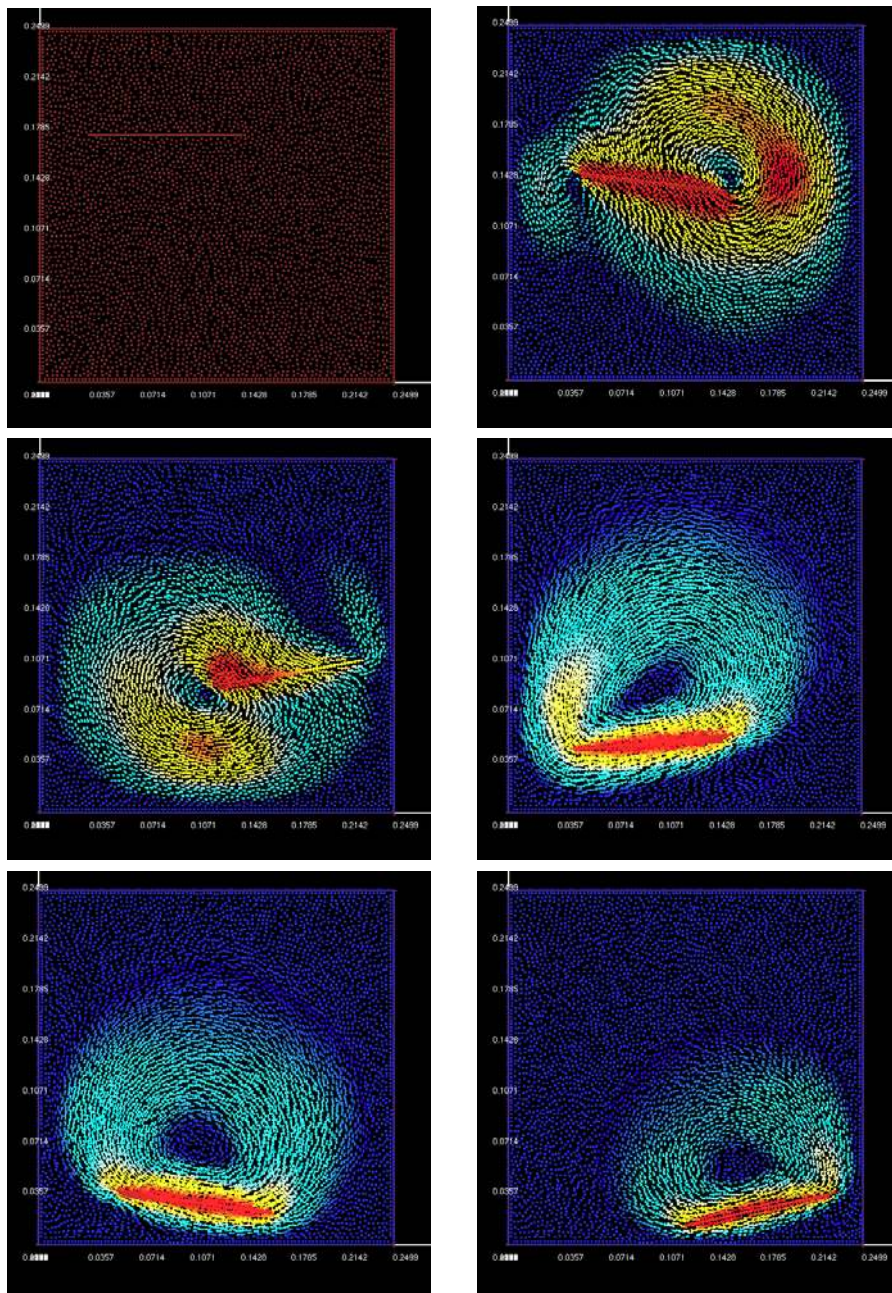
Figure 4. Velocity field at t = 0.0, 0.3 s (top), t = 0.6, 0.9 s (center) and t = 1.2, 1.5 s (bottom)
