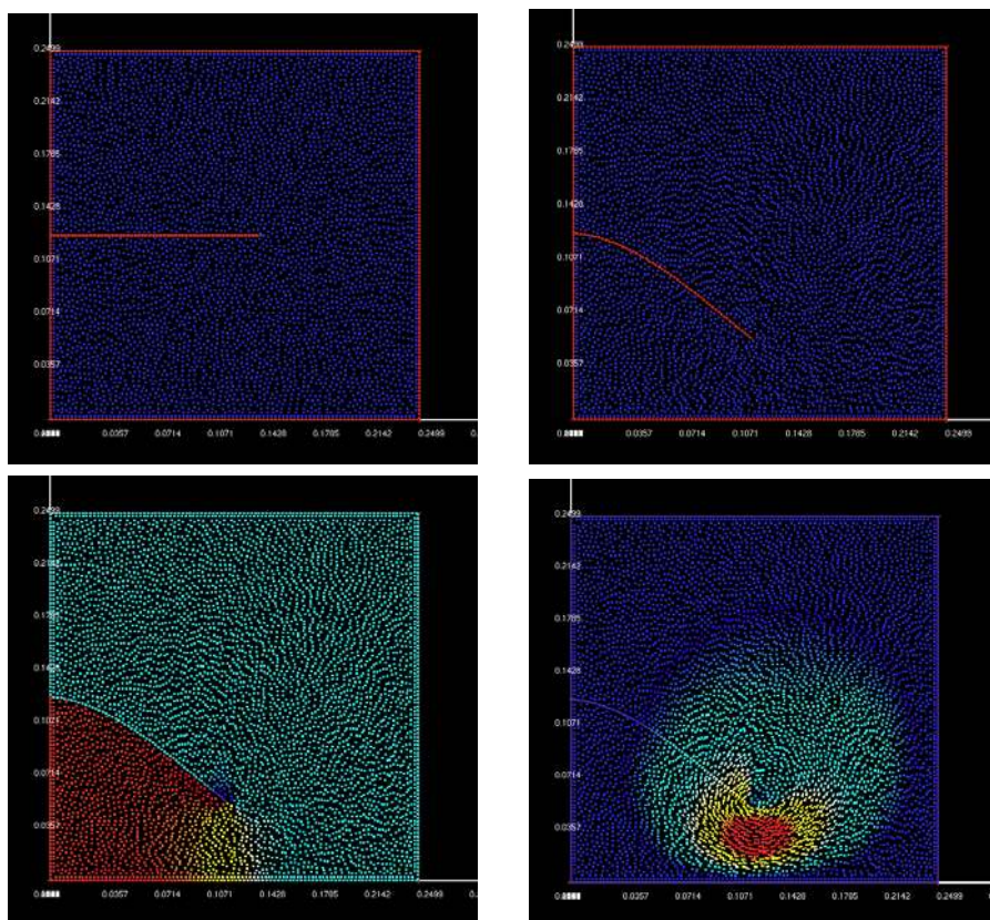
Figure 2. Position of particles and sheet of paper at time t = 0 s and t = 0.8377 s (top), pressure and velocity field at t = 0.8377 s (bottom)
