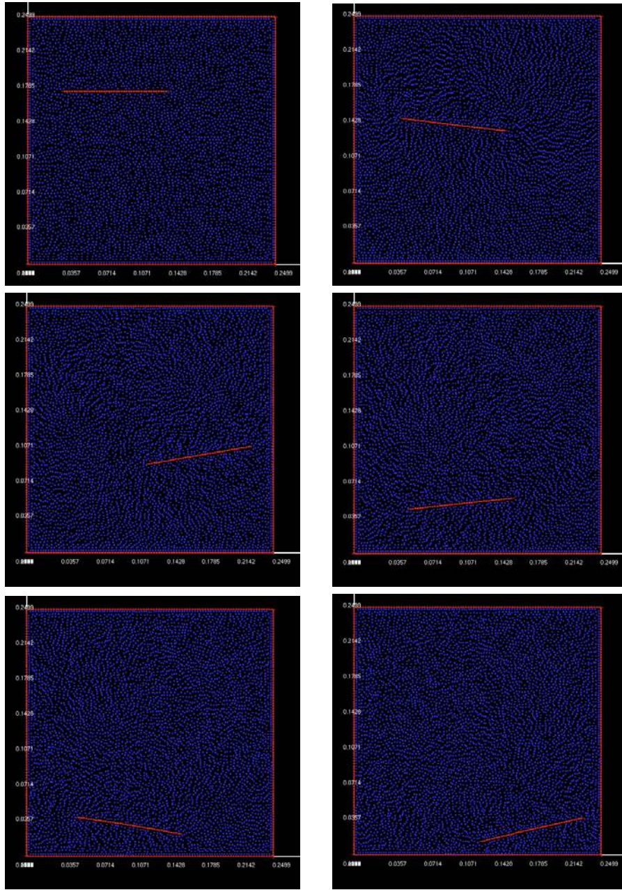
Figure 3. Position of particles and sheet of paper at t = 0.0, 0.3 s (top), t = 0.6, 0.9 s (center) and t = 1.2, 1.5 s (bottom)
