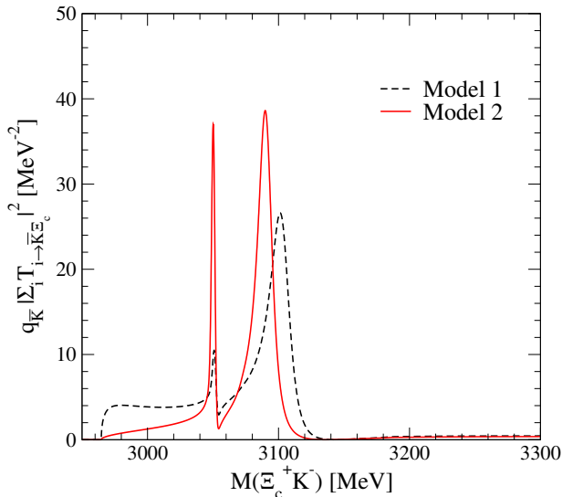
FIG. 4: (Color online) Sum of amplitudes squared times a phase space factor.
