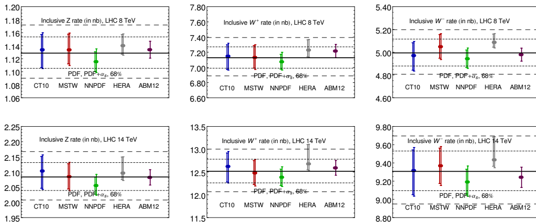
Figure 20. Comparison of inclusive W^\pm and Z cross sections at NNLO for various PDF ensembles. The PDF and PDF+ \alpha_s errors of META PDFs (at 68% c.l.) are shown by the short-dashed and long-dashed lines.
