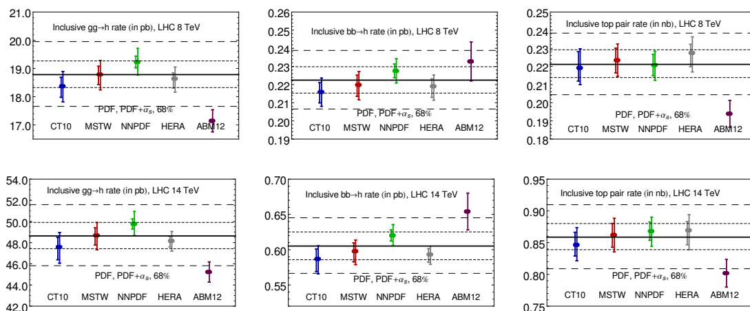
Figure 21. Comparison of inclusive Higgs boson and top quark pair production cross sections at NNLO for various PDF ensembles. The PDF and PDF+ \alpha_s errors of META PDFs (at 68% c.l.) are shown by the short-dashed and long-dashed lines.
