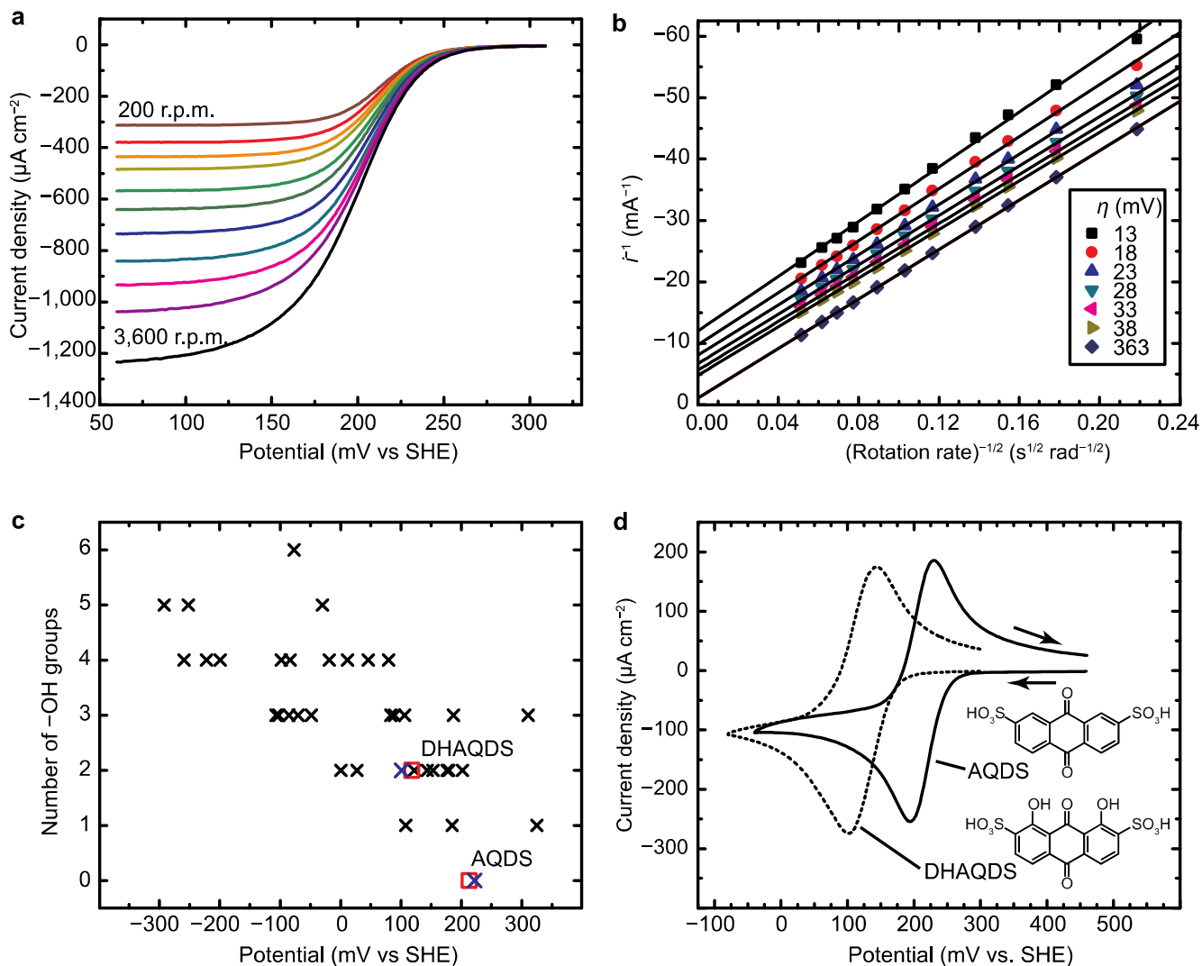
Figure 3 | Half-cell measurements and theory calculations. a , Rotating disk electrode (RDE) measurements of AQDS using a glassy carbon electrode in 1 M \text{H}_2\text{SO}_4 at 11 rotation rates ranging from 200 r.p.m. (red) to 3,600 r.p.m. (black). b , Koutecký-Levich plot (current ^{-1} versus rotation rate ^{-1/2} ) derived from a at seven different AQDS reduction overpotentials, \eta . c , Calculated reduction potentials of AQDS substituted with -OH groups (black), calculated AQDS and DHAQDS values (blue), and experimental values for AQDS and DHAQDS (red squares). d , Cyclic voltammogram of AQDS and DHAQDS (1 mM) in 1 M \text{H}_2\text{SO}_4 on a glassy carbon electrode (scan rate = 25 \text{mV s}^{-1} ).
