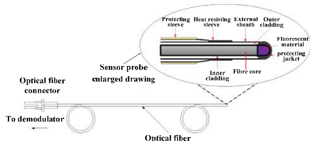
FIGURE 2. Optical fiber temperature sensor.
