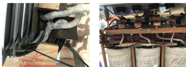
FIGURE 3. Optical fiber temperature sensors arrangement in temperature rise test.
