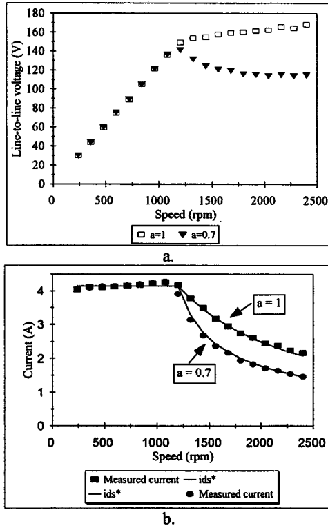
Fig. 3. Measured fundamental components of stator voltage (a) and stator no-load current (b), for b = 7 and two values of parameter a (stator d-axis current reference rms values included in (b)).
