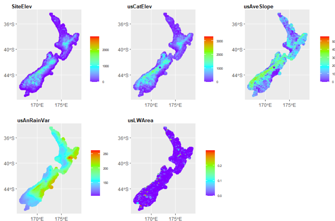
Figure A2. Spatial distribution of the five environmental variables used in regression kriging of residuals (Eq. 3). Except for SiteElev, all other factors are averaged across the upstream catchments.
