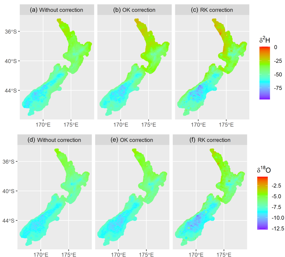
Figure 6. Predicted \delta^2\text{H} and \delta^{18}\text{O} of surface water of New Zealand. Panels (a) and (d) show uncorrected values from the water balance model. Panels (b) and (e) give residual-corrected values based on ordinary kriging (OK correction). Panels (c) and (f) give residual-corrected values based on regression kriging (RK correction).
