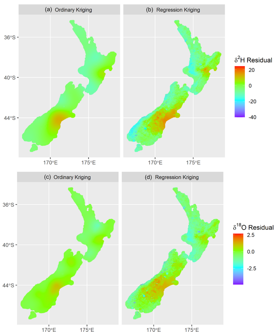
Figure 4. Distribution of isotope residuals (i.e. difference between modelled and observed isotopes) from ordinary kriging (a, c) and regression kriging (b, d). Positive values equate to a negative adjustment of river \delta^2\text{H} and \delta^{18}\text{O} values from the water balance model, as seen in leeward (eastern) areas of both the North and South islands. Ordinary kriging results in regional zones of negative isotope residuals around validation sites downstream from lakes and wetlands (such as in the central North Island), while regression kriging predicts negative isotope residuals in low-elevation western areas and in all lakes and wetlands and their downstream reaches.
