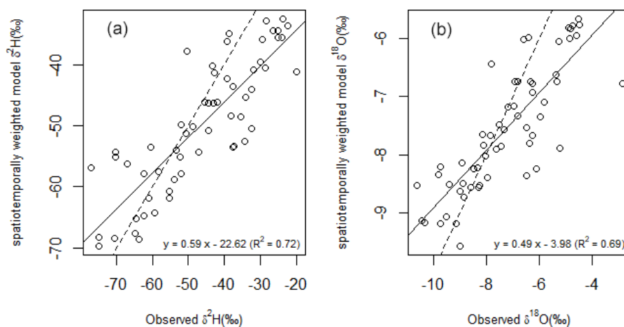
Figure 2. Relationship between modelled and observed \delta^2\text{H} (a) and \delta^{18}\text{O} (b) at 58 long-term river water monitoring sites across New Zealand. Modelled isotopes were the long-term averages of simulated isotopes computed following the water balance model approach of Bowen et al. (2011). The solid line shows the regression fit, and the dashed line shows a 1 : 1 fit. The modelled values tend to overpredict the river water isotope at the more negative end of the range (e.g. at high-latitude cooler southern sites) and underpredict at the less negative end of the range (e.g. warmer, northern sites).
