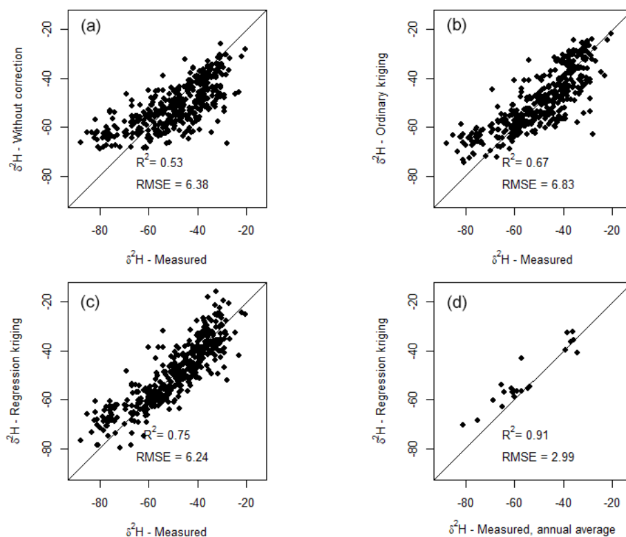
Figure 5. Comparison of the literature values of water \delta^2\text{H} across New Zealand rivers, with predicted long-term average \delta^2\text{H} values from the uncorrected water balance model (a), ordinary-kriging-corrected model (b), and regression-kriging-corrected model (c). Panel (d) shows a comparison between predictions of the regression-kriging-corrected model with mean annual measured values at sites with > 1 year of monthly data. Lines show a 1 : 1 relationship.
