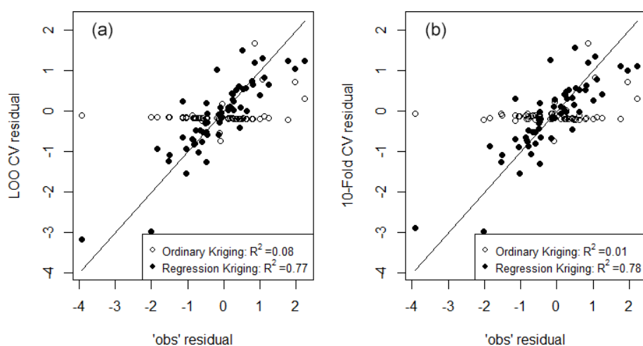
Figure 3. Comparison between observed residuals and spatial predictions of residuals made using two interpolation methods, i.e. ordinary kriging and regression kriging. Observed residuals are the differences between spatiotemporal model predictions of \delta^{18}\text{O} and measurements from 58 long-term river monitoring sites across New Zealand. Comparison with estimates of residuals generated using the LOOCV (a) and 10-fold cross-validation (b) suggests the improved fit of regression kriging relative to ordinary kriging.
