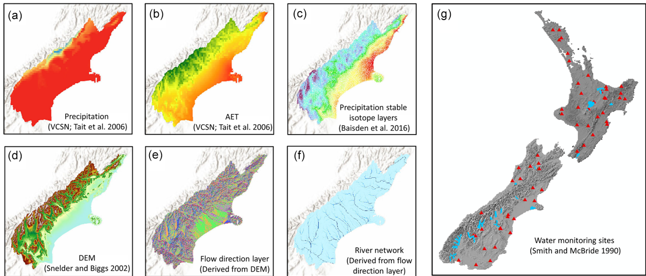
Figure 1. GIS layers and data sources used in model development. Panels (a)–(f) show GIS layers used for water balance modelling, plotted over the Canterbury region in New Zealand's South Island. Precipitation, actual evapotranspiration (AET), and stable isotope values of precipitation (a–c) are used to calculate catchment-scale, flow-weighted isotope values of recharge ( \delta Q ; i.e. flow \times isotope \delta value). The river network (f) is derived from the DEM (d) and flow direction (e) layers by setting a suitable flow accumulation threshold. Catchment \delta Q values are routed downstream through the river network to generate reach-scale estimates of \delta^2\text{H} and \delta^{18}\text{O} . Panel (g) shows river water isotope measurement sites (triangles) used for model correction and major lakes (blue area).
