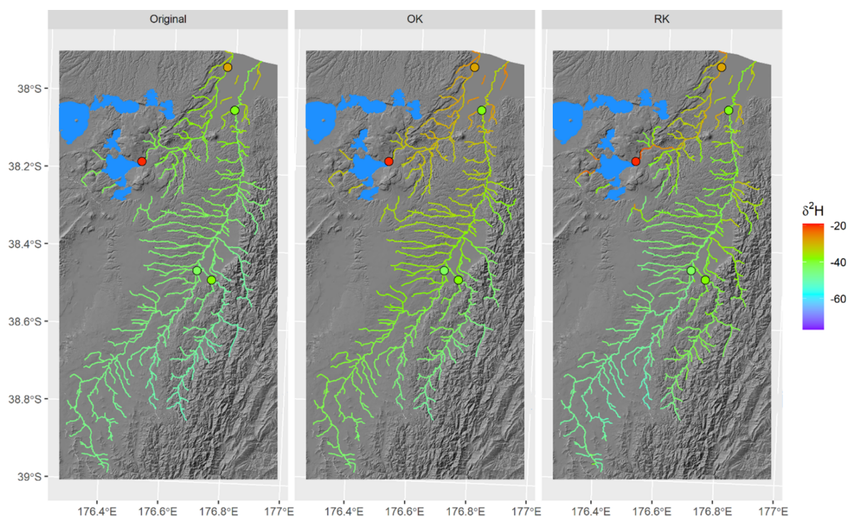
Figure 7. Comparison of modelled \delta^2\text{H} values of river water across two neighbouring North Island basins (Tarawera and Rangitaiki basins). Higher \delta^2\text{H} values from ^2\text{H} -enriched precipitation lower in these catchments are represented by the water balance model (original). Residual correction using ordinary kriging (OK) extends the enrichment effect of Lake Tarawera (top left of each panel) across the entire region. Using regression kriging (RK), the lake enrichment is mostly confined to downstream reaches. Points denote the locations and observed \delta^2\text{H} values at the gauging sites.
