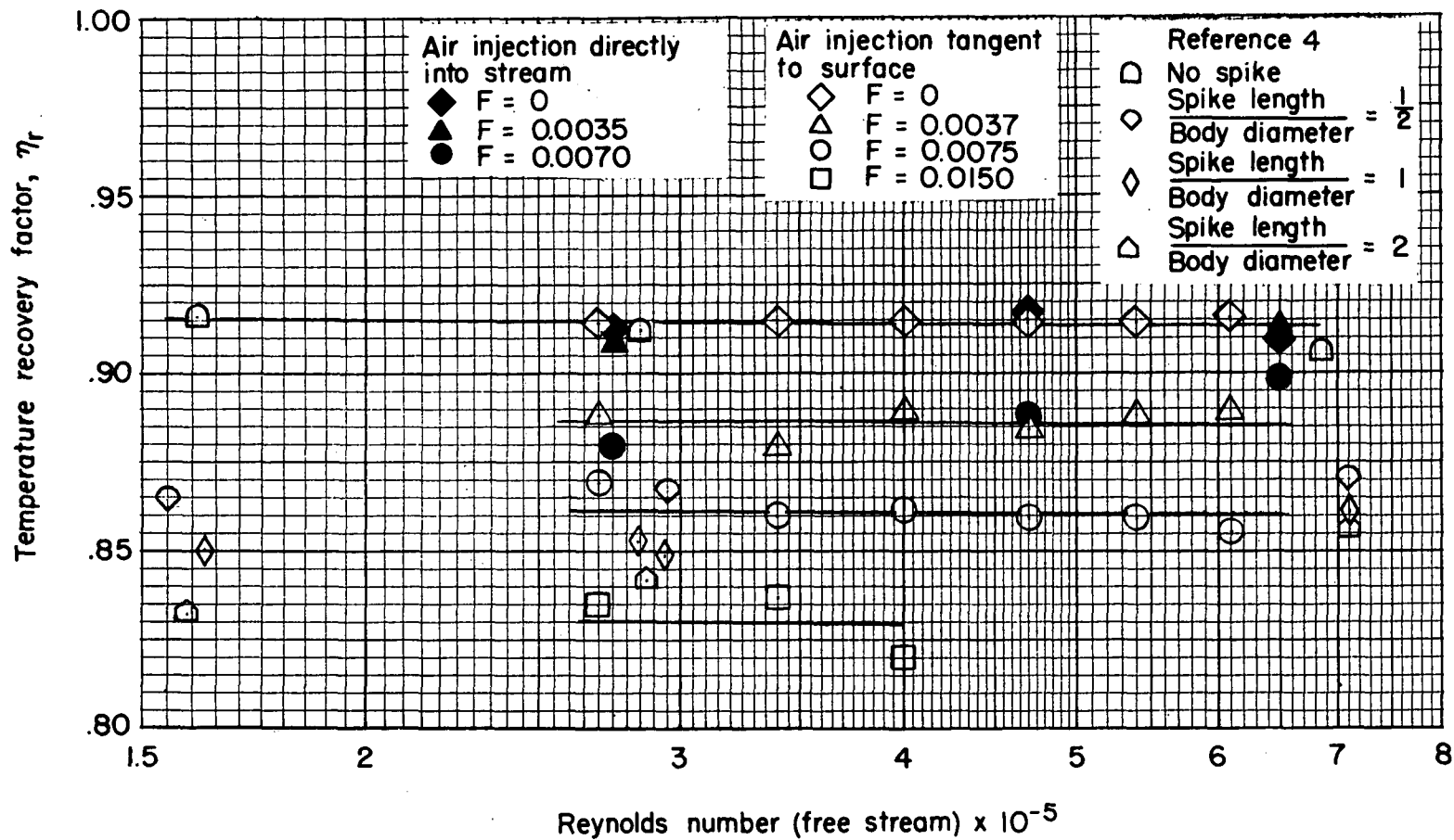
Figure 4.- Average temperature recovery factor for hemispherical nose with, and without, air injection.
