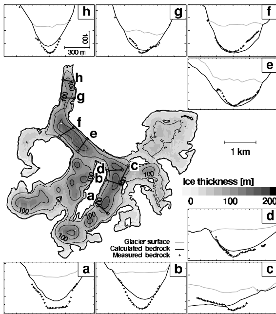
Fig. 7. Calculated ice-thickness distribution of Glacier de Zinal. The insets (a–h) show the marked cross-sections; all have the same vertical exaggeration.
