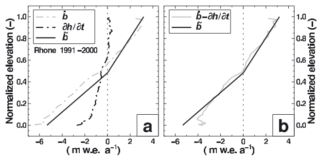
Fig. 11. Altitudinal distribution of modelled mass balance \hat{b} , observed rate of ice-thickness change \partial h/\partial t (Huss and others, 2008a) and estimated apparent mass balance \tilde{b} (a) and difference \hat{b} - \partial h/\partial t and estimated \tilde{b} (b) for Rhonegletscher. The elevation range is normalized. Values are means over the period 1991–2000 and expressed in \text{m w.e. a}^{-1} .
