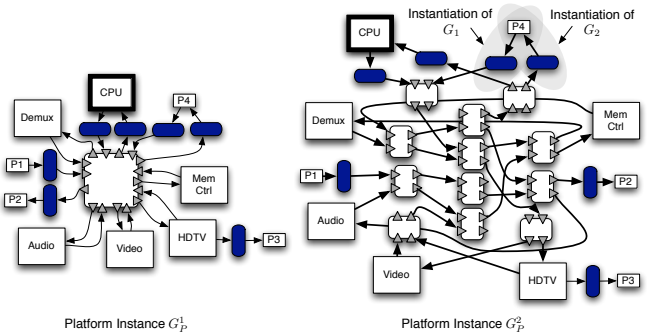
Fig. 3. Two NoC instances obtained by instantiation and composition of communication components.
