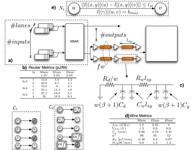
Fig. 7. Modeling the NoC components.
