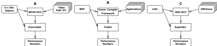
Fig. 10. Y-chart environments used in various design projects.
