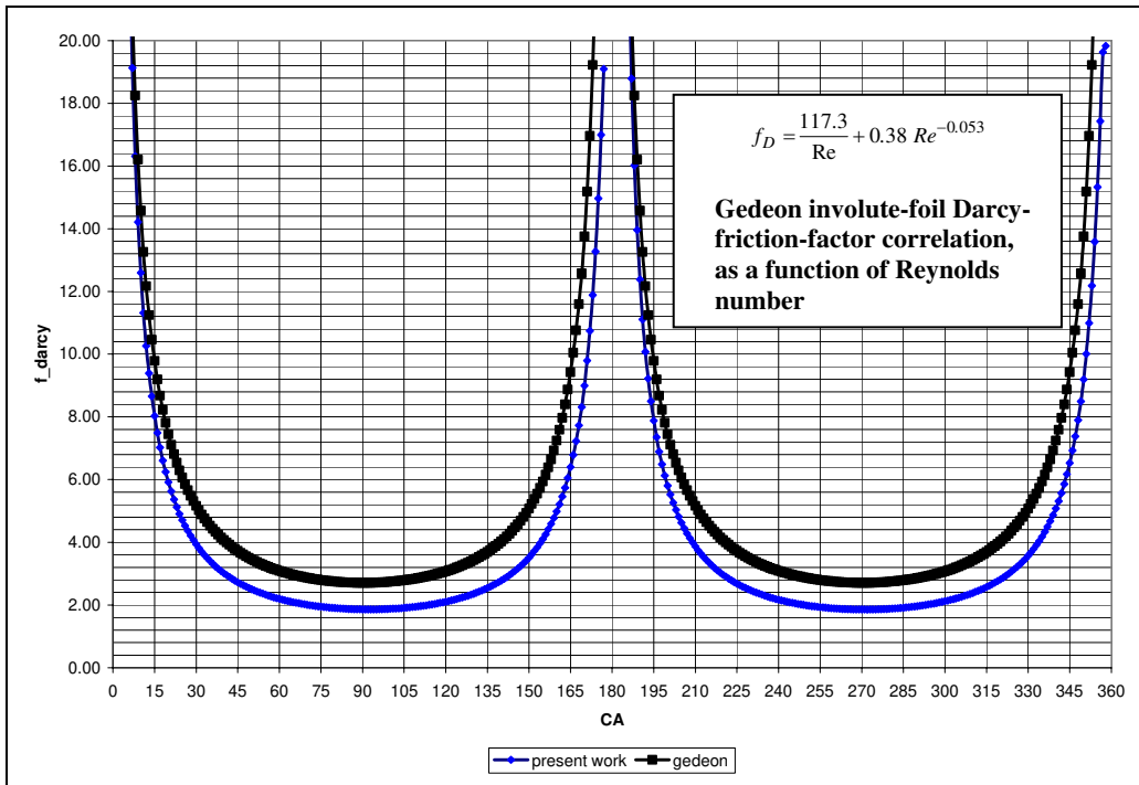
Figure 29.—Darcy friction factors, f_{Darcy} , as functions of crank angle, CA , degrees; comparisons of values calculated from 2-D CFD base-oscillatory-flow case (50 by 20 grids/segment) with Gedeon involute-foil test-data correlation; this test-data correlation is shown on the figure in the form of Darcy friction-factor as a function of Reynolds number.
