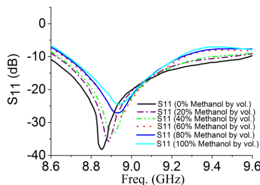
Fig. 7 Measured S_{11} plot for Methanol and DI water mixtures.
