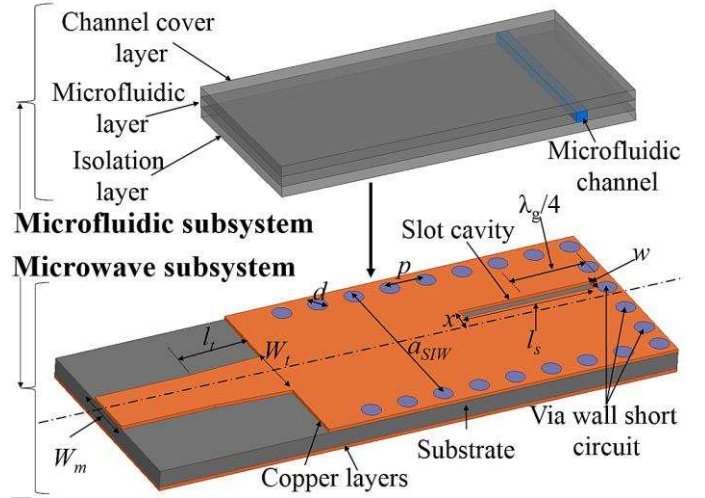
Fig. 1. 3D drawing of SIW waveguide integrated with a single slot antenna and microfluidic subsystem.
