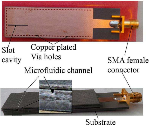
Fig.2 Fabricated prototype, before (top) and after (bottom) mounting the microfluidic subsystem.
