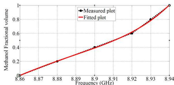
Fig.8 Methanol fractional volume against resonant frequency.
