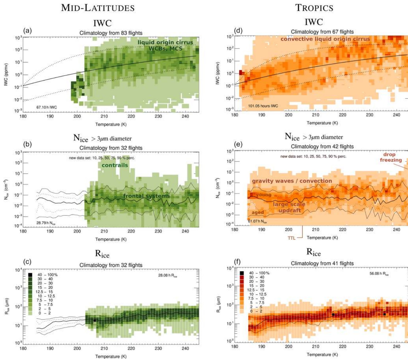
Figure 8. Same as Fig. 7a–c, but for midlatitudes and tropics (WCBs: warm conveyor belts; MCS: mesoscale convective systems; TTL: tropical tropopause layer). The field campaigns are listed in Table A2.
