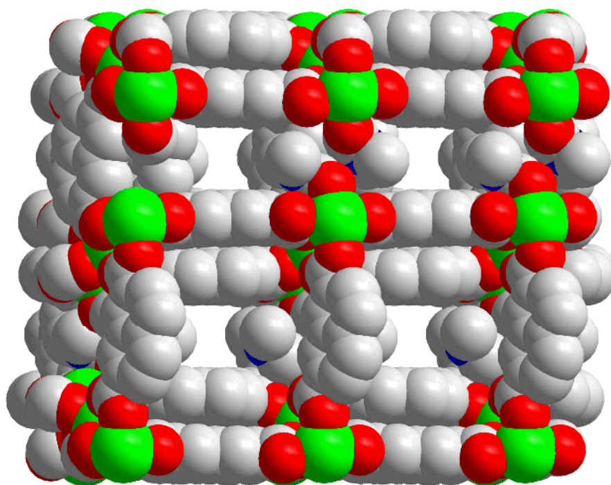
Figure S2. CPK drawing of 1 .
