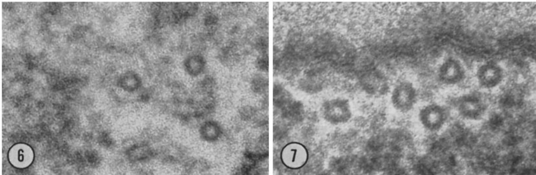
FIGURE 6 Cross-section through metaphase spindle of Spirodela , showing three tubules with an outside diameter of about 230 A. A small part of a chromosome is included at the left. \times 240,000 .
