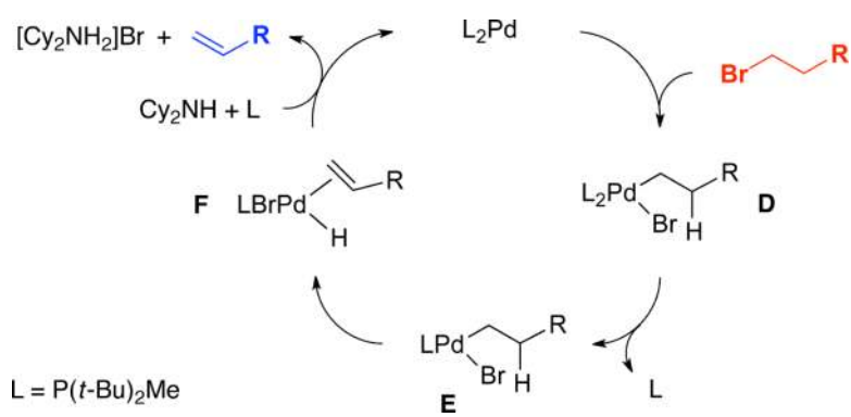
Figure 3. Outline of a possible mechanism for Pd(P(t-Bu)_2Me)_2 -catalyzed dehydrobromination reactions.
