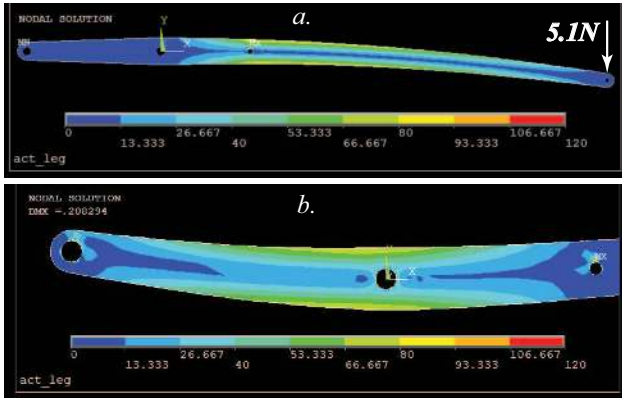
Fig. 7. Results of the FEA on a simplified 2D model of the main leg. a. Stress at take-off, max. von Mises stress \sigma_m \approx 90 MPa , max. deflection d = 0.9mm . b. Stress in charged position, max. von Mises stress \sigma_m \approx 85 MPa , max. deflection d = 0.21mm .
