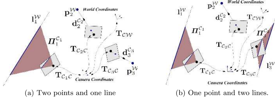
Fig. 1: Illustration of the two minimal problems solved in this paper. We estimate the transformation parameters \mathbf{T}_{CW} in two different settings: the case where we have two 3D points, one 3D line, and their respective images (a); and the case where we have two 3D lines, one 3D point and their respective images (b).
