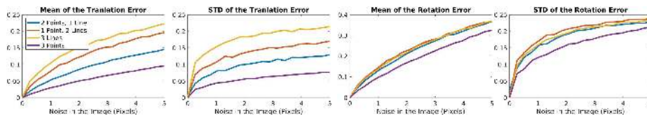
Fig. 4: Comparative results for the methods using different type of features, as a function of the noise in the image pixels. 2 Points, 1 Line and 1 Point, 2 Lines show the results for the methods presented in this paper, while 3 Points and lines 3 Lines are techniques proposed in [10,11].
