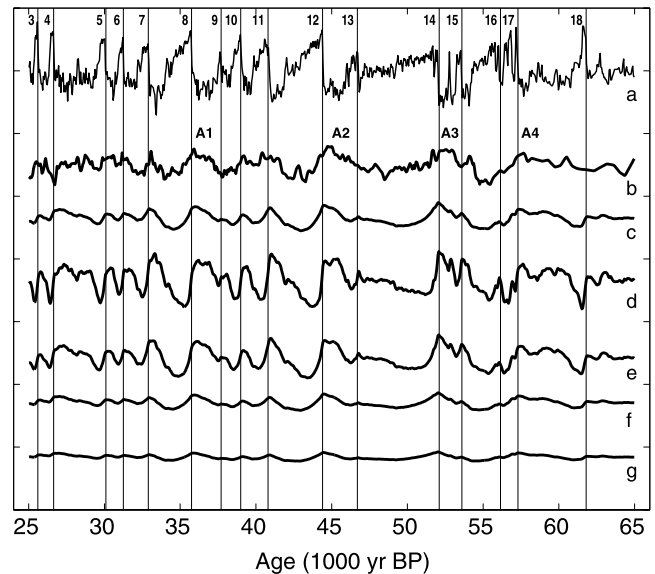
Figure 5. Filtered isotopic data from GRIP (curve a) and Byrd (curve b) using a high-pass filter with a cutoff at 8000 years to remove Milankovic timescales for which the bipolar seesaw does not apply. Modeled time series of Byrd according to equation (2) are given for \tau = 1120 years (curve c), for \tau = 200 years (curve d), for \tau = 500 years (curve e), for \tau = 2000 years (curve f), and for \tau = 4000 years (curve g), using the filtered GRIP record as input and the characteristic timescale \tau . Using the characteristic timescale \tau = 1120 years (curve c) yields the highest correlation with the filtered Byrd data (curve b). The other model realizations (curves d–g) with shorter or longer timescales show less agreement with Byrd. The vertical lines mark the Dansgaard/Oeschger events in GRIP. Antarctic warmings in addition to the classic warmings A1 to A4 can be identified.
