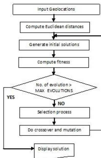
Fig. 2 Block Diagram of the Genetic Algorithm Implementation
