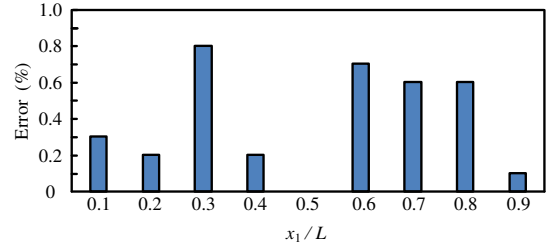
Fig. 12 Location errors of different short-circuit fault points.
