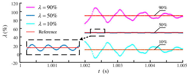
Fig. 5 The calculated \lambda for different fault locations.
